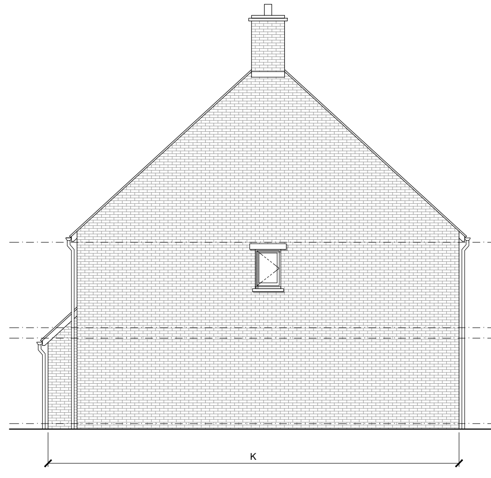
Side Elevation - K 1:100 (A3)
