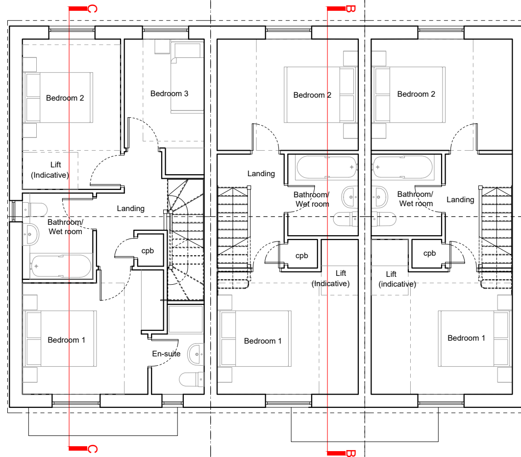
First Floor Plan - BKK 1:100 (A3)
