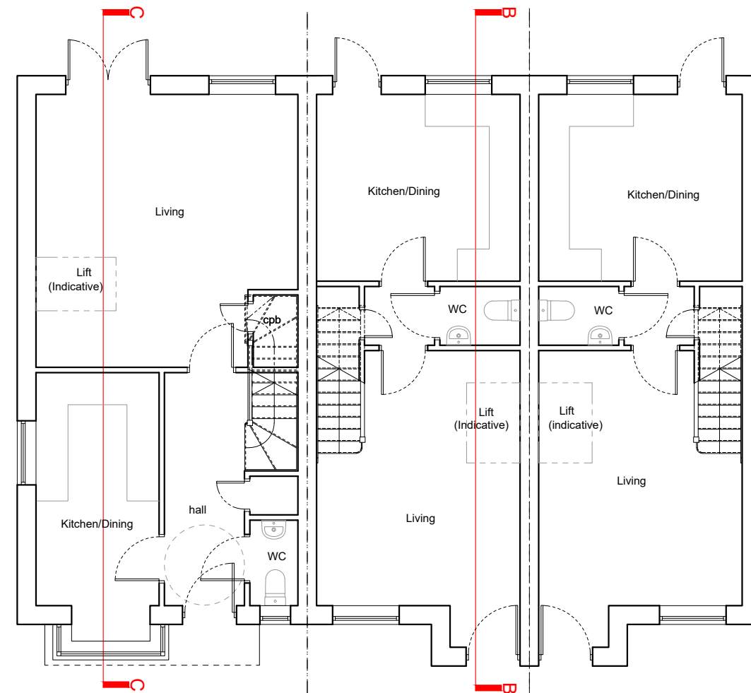
Ground Floor Plan - BKK 1:100 (A3)
