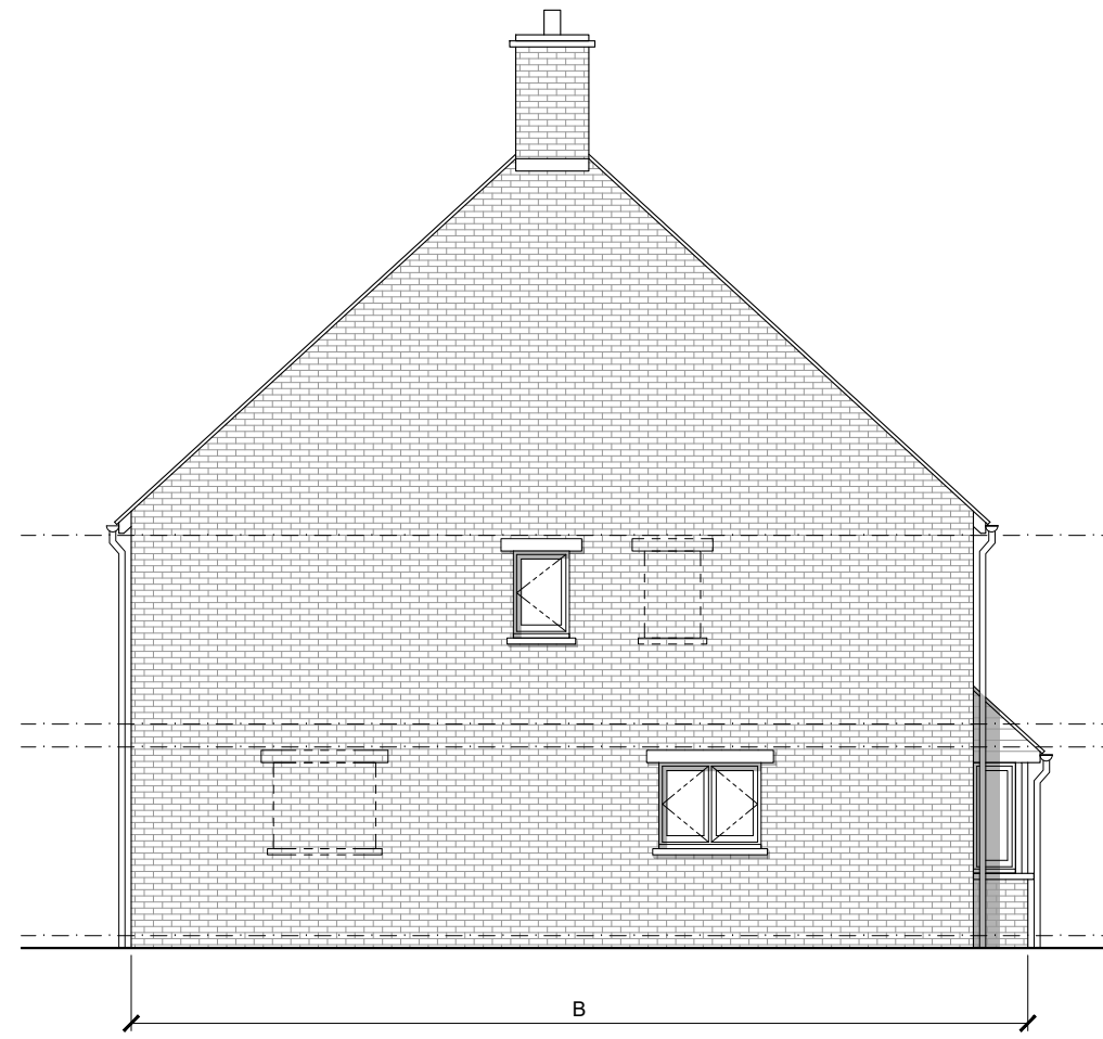
Side Elevation - B 1:100 (A3)
