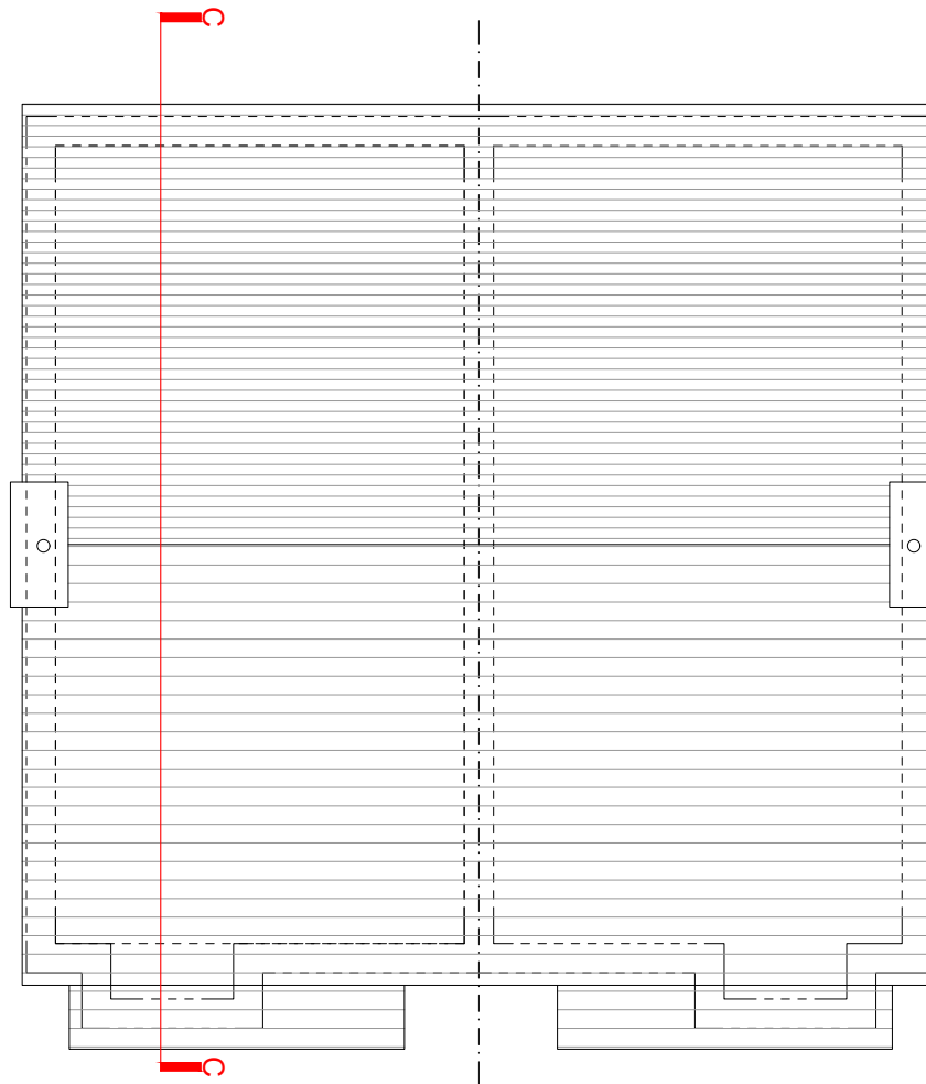
Roof Plan - BB 1:100 (A3)
