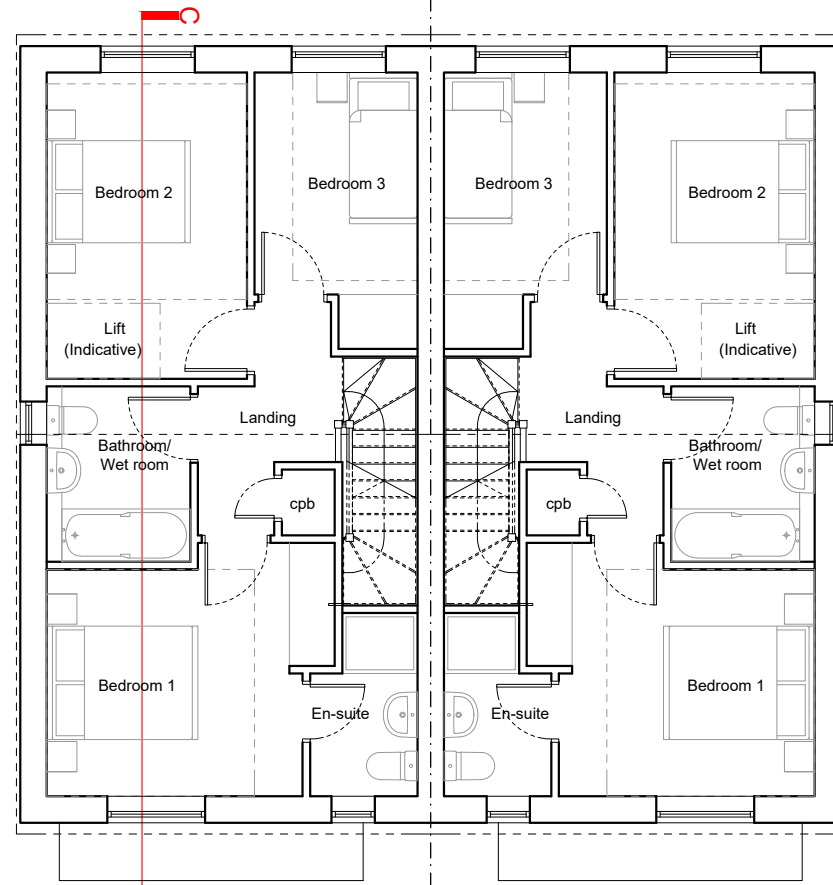
First Floor Plan - BB 1:100 (A3)
