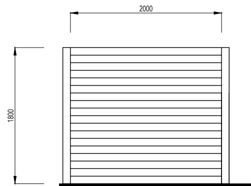
Plot Division Panel Fence 1800mm High
