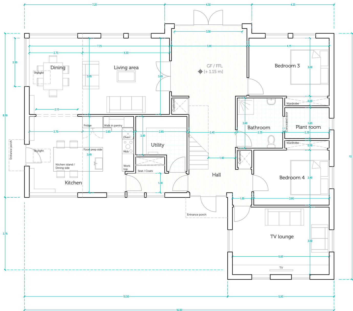
Ground floor 161.6 m 2
