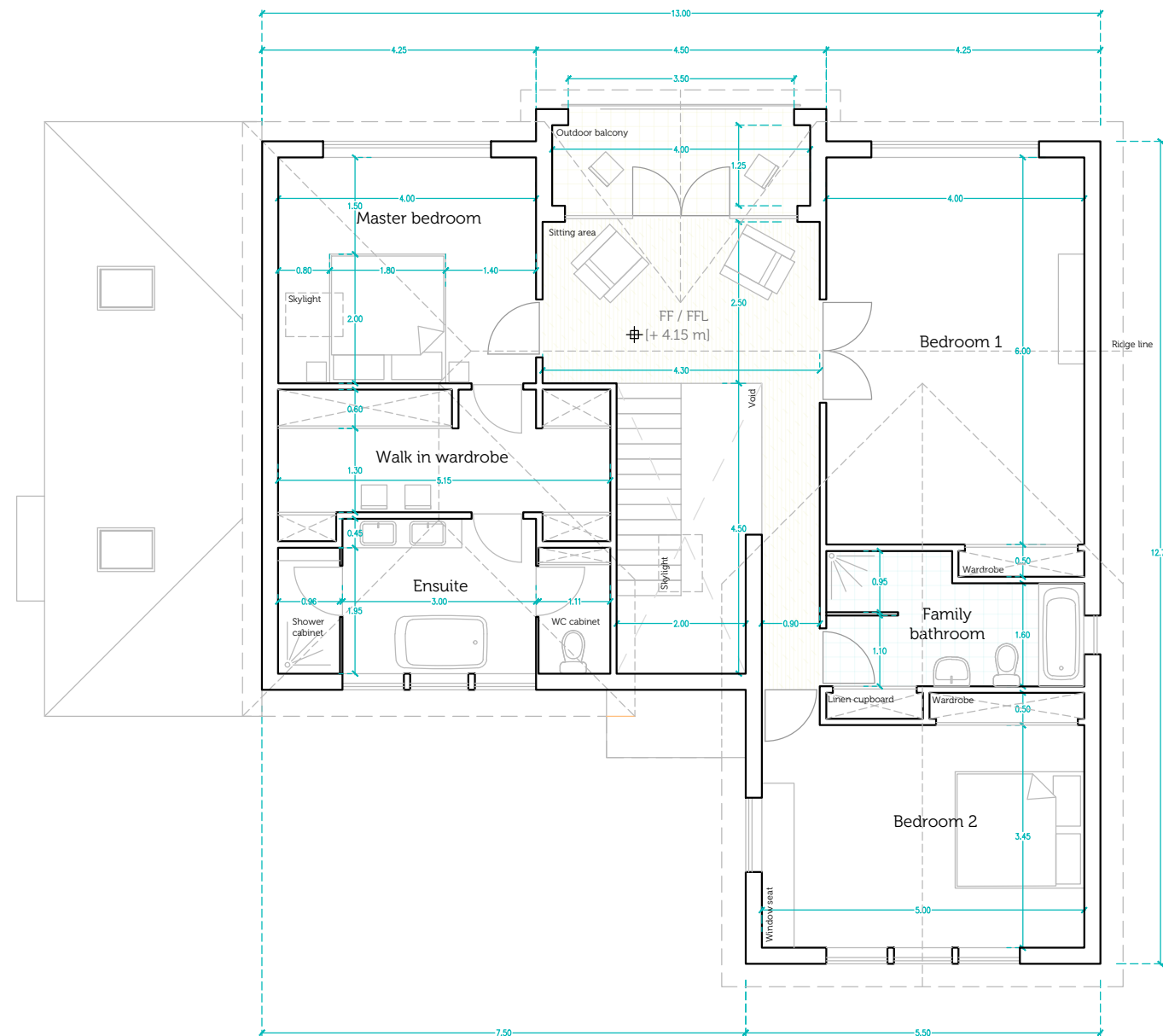
First floor 136.15 m 2
