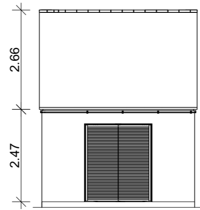
Front Elevation
