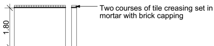
F2 1800mm Brick Screen Wall
