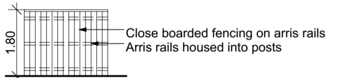
F1 1800mm Close boarded fence
