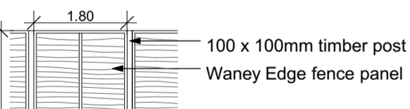
F3 1800mm high Waney Edge fence
