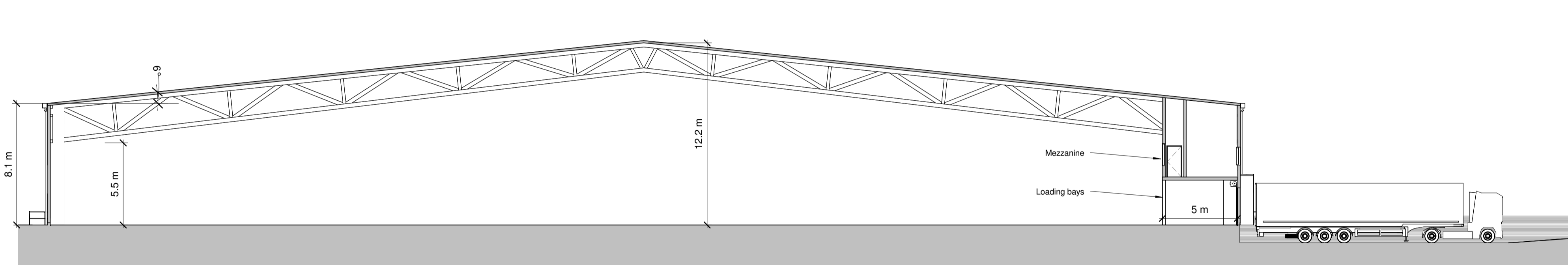
2 | P-14 - Section 2 - Phase 1 1:200
