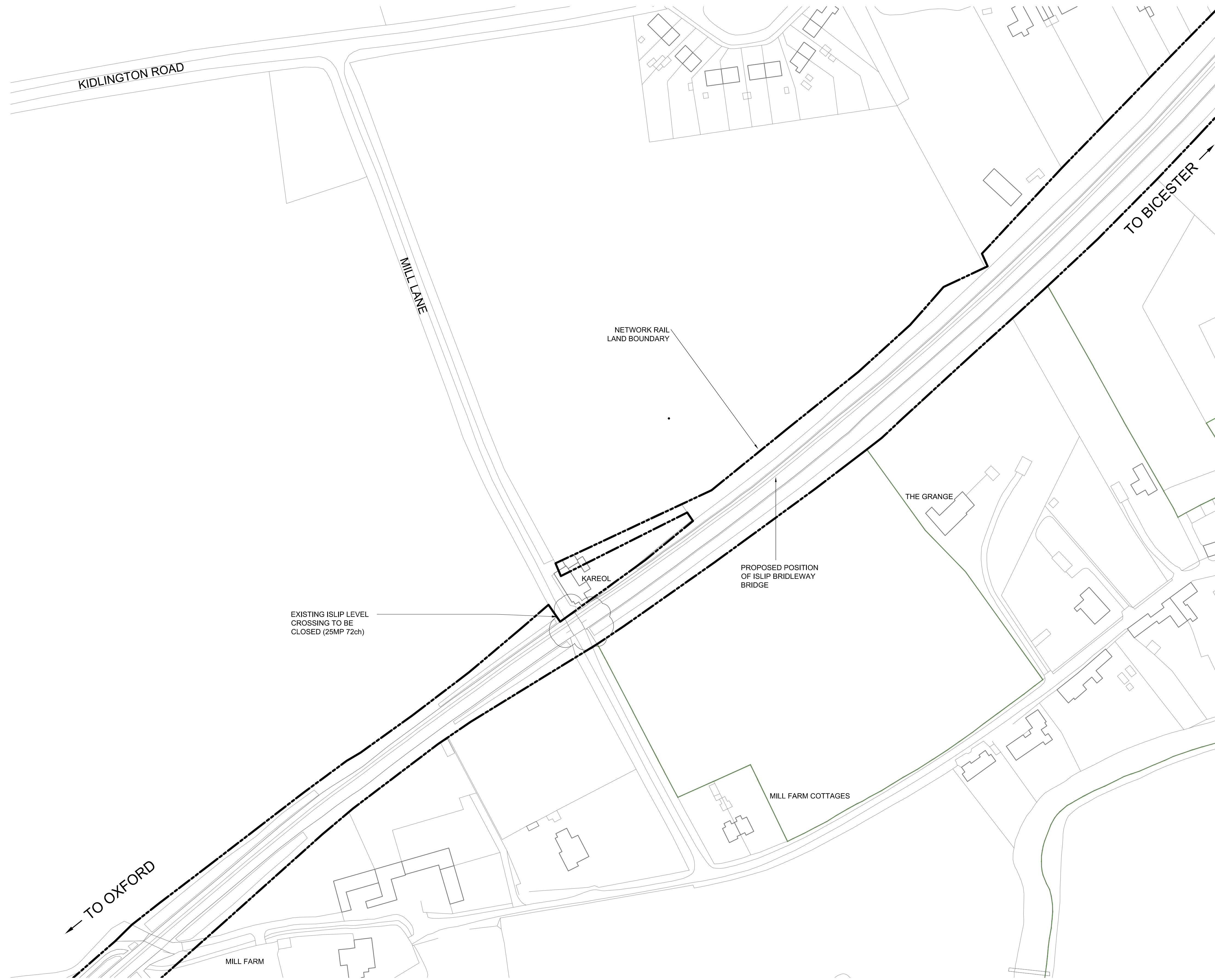
LAND BOUNDARY PLAN 1:1000 0 20 40 60 80 100m SCALE 1:1000
