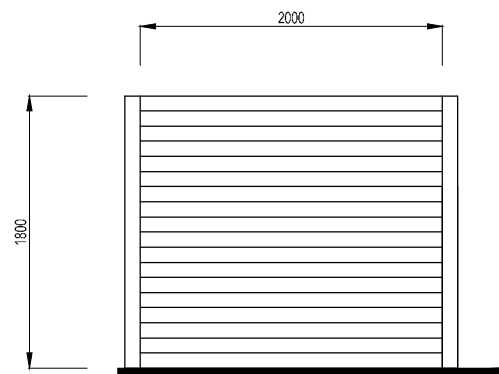
1800mm High Plot Division Panel Fence
