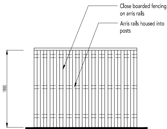
1800mm High Close Board Fence
