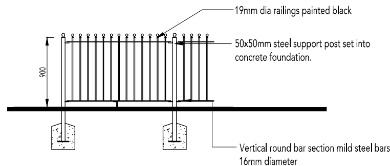
900mm High Estate Railings
