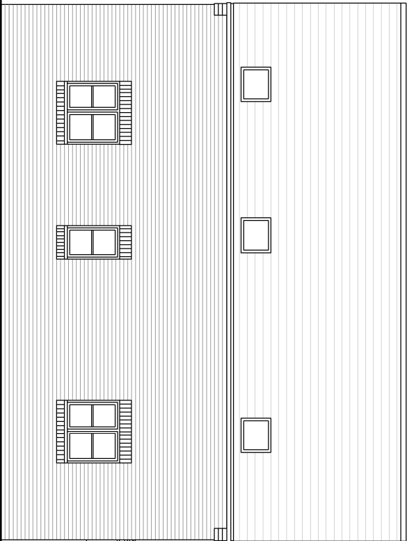
REAR ELEVATION
