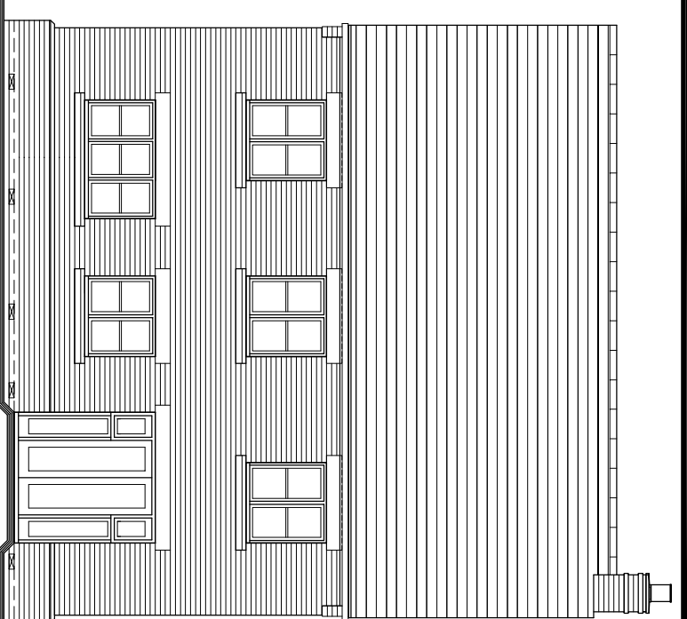
REAR ELEVATION
