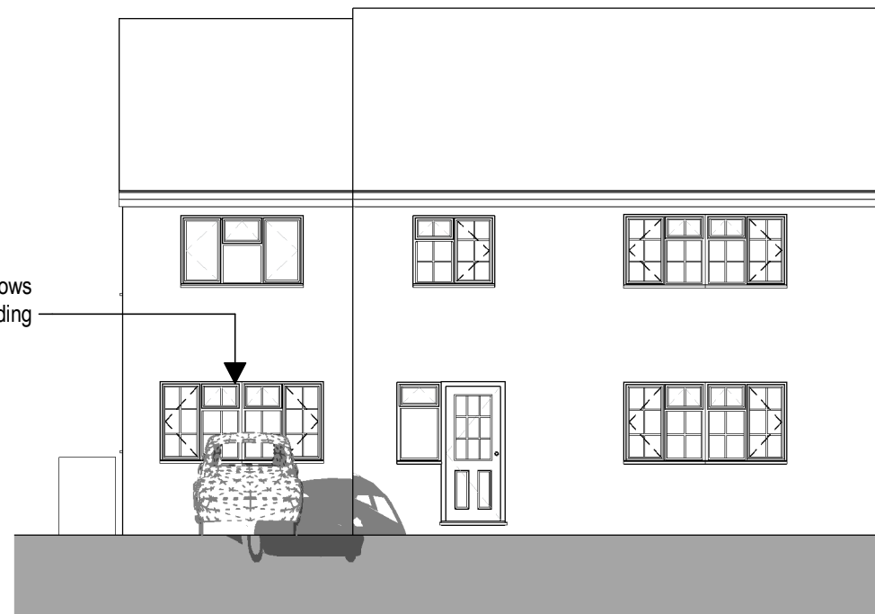
4 3201 West Elevation 1 : 100
