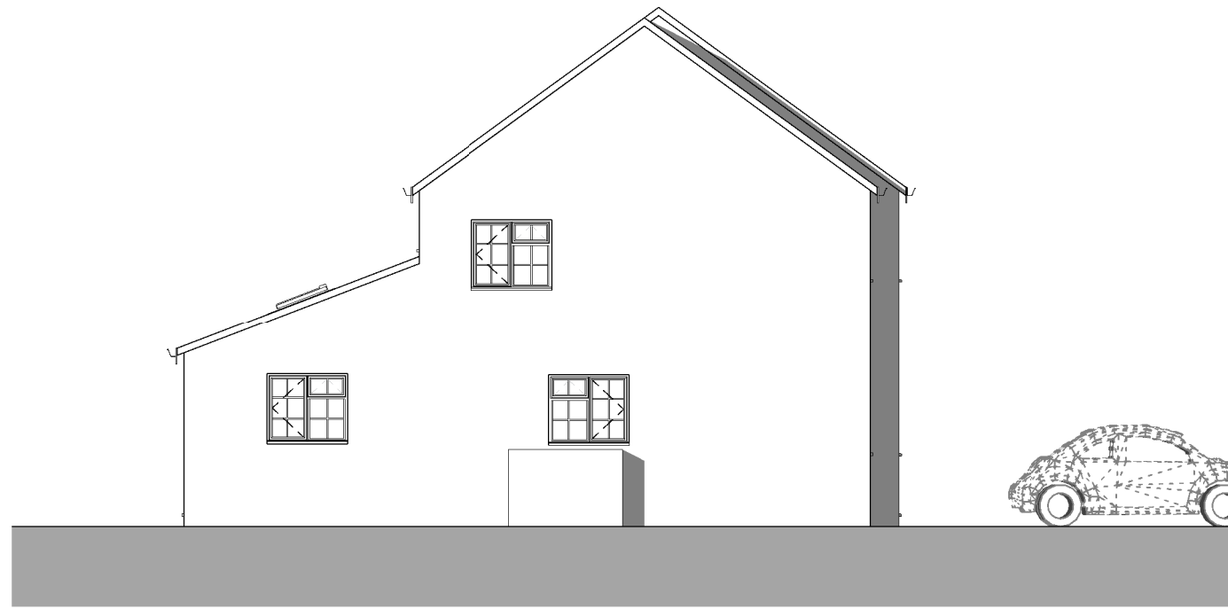
1 3201 North Elevation 1 : 100
