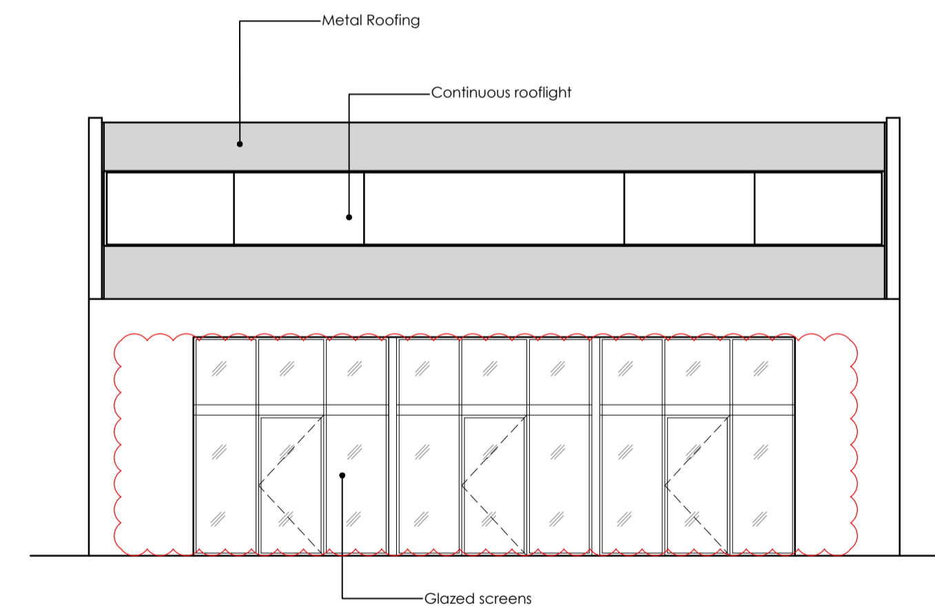
BUILDING 104 SOUTH EAST ELEVATION - PROPOSED
