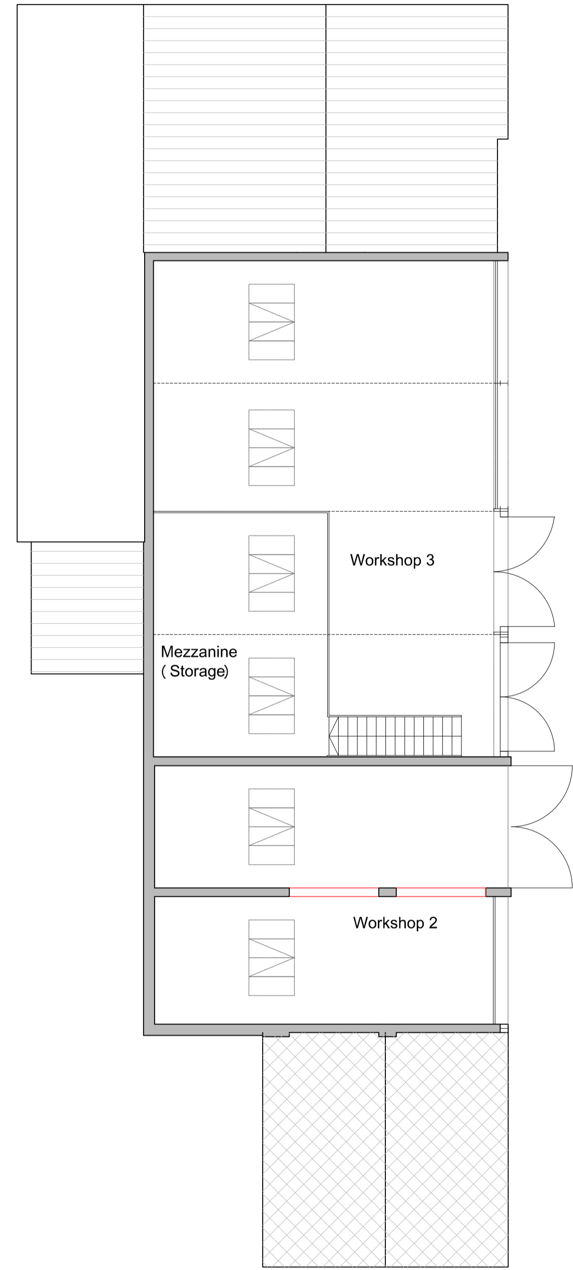
BUILDING 131 Mezzanine Floor Plan - Proposed
