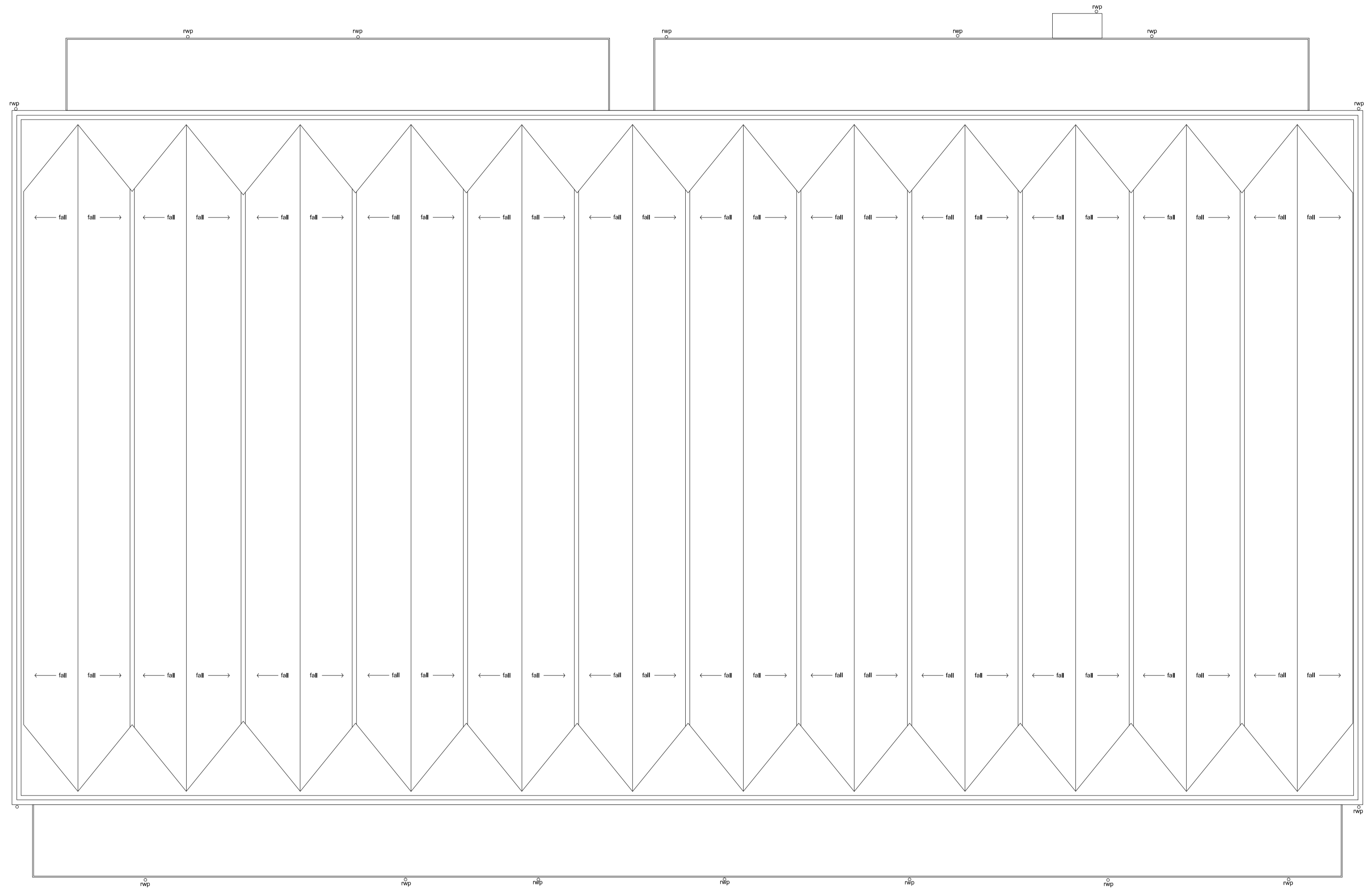
BUILDING 113 Roof Plan-Existing (assumed only)
