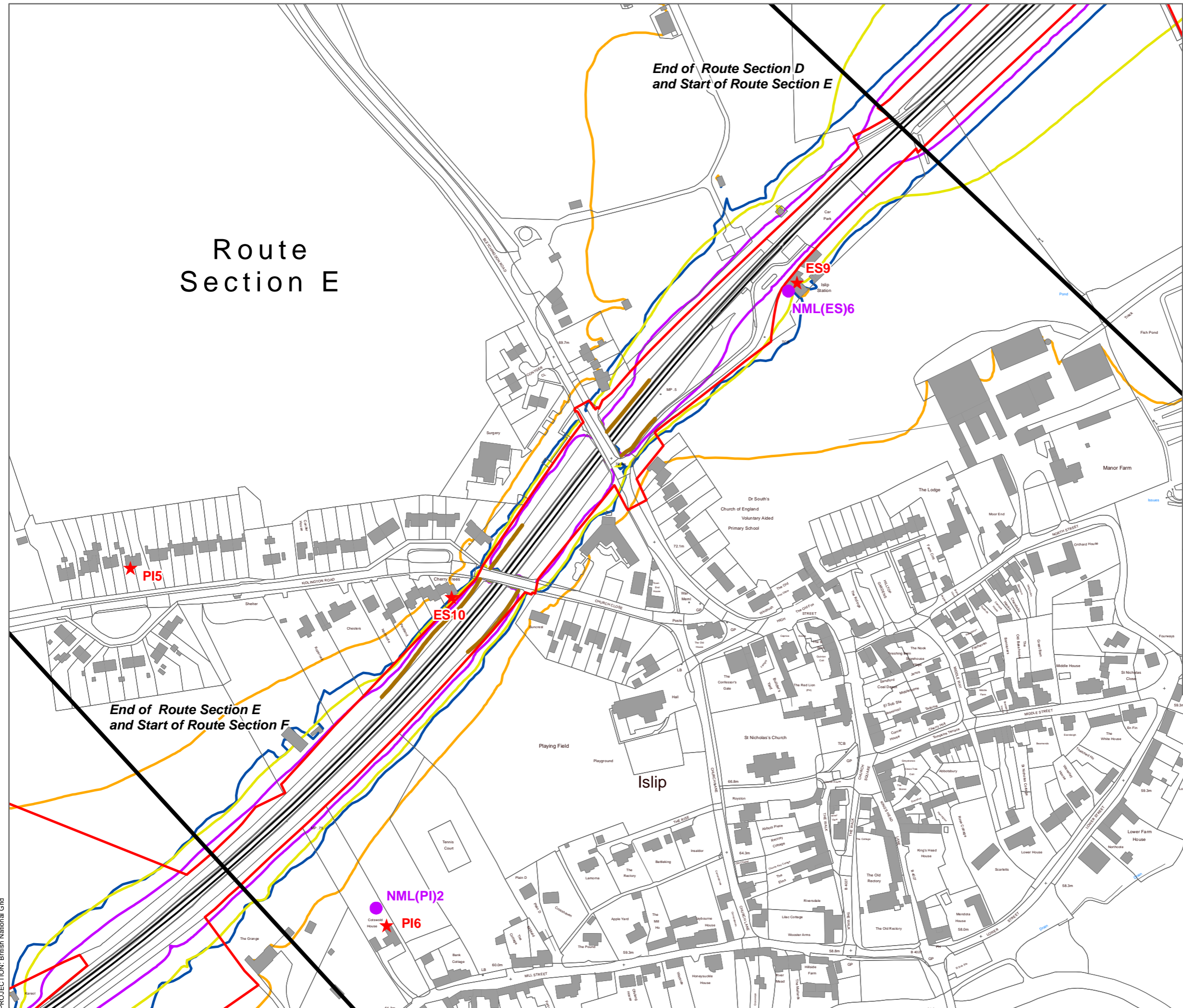
Figure 5.1 Location of Noise Barriers, Noise Contours Showing Extent of Noise Insulation and Residual Noise Levels from the Order Scheme
