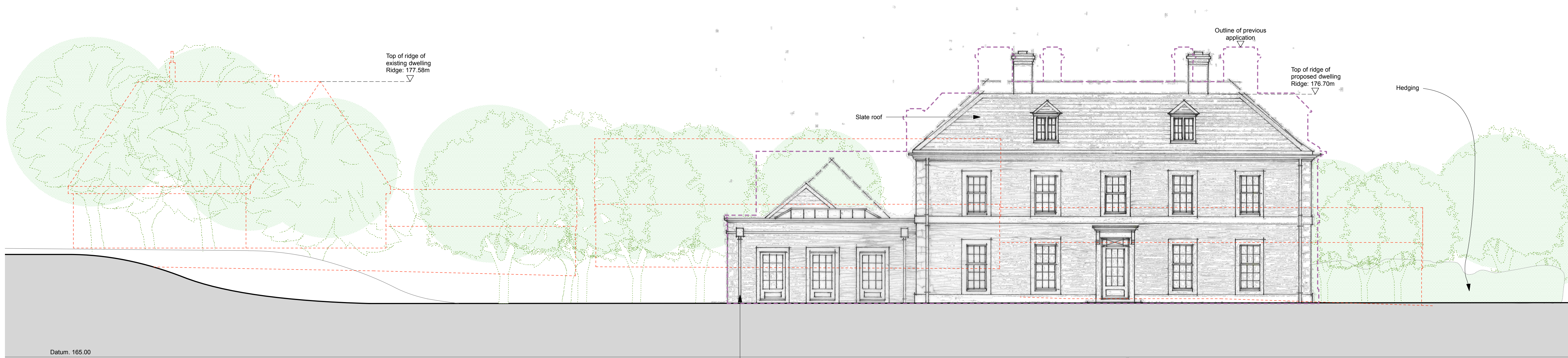
3: West Elevation
