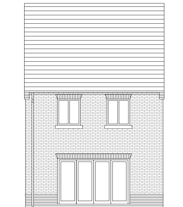
REAR ELEVATION
