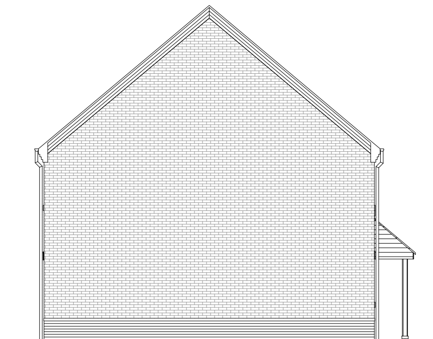
LEFT ELEVATION
