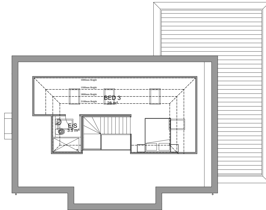
SECOND FLOOR
