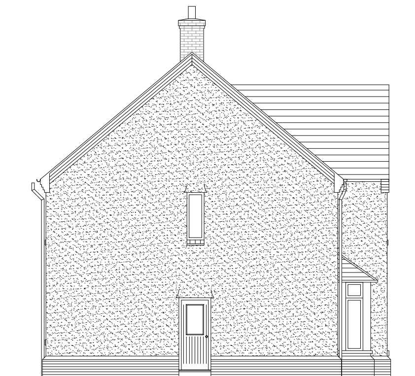
LEFT ELEVATION
