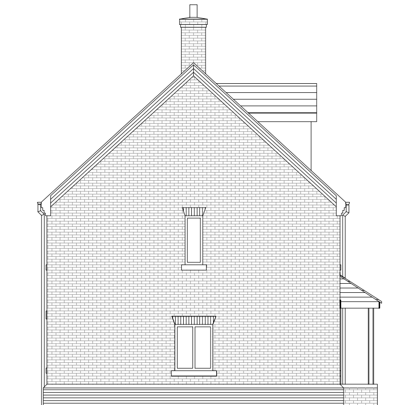
LEFT ELEVATION
