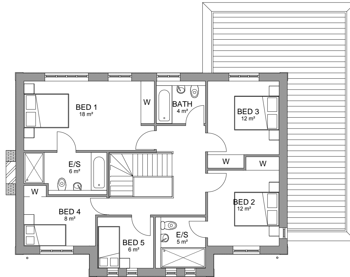
FIRST FLOOR
