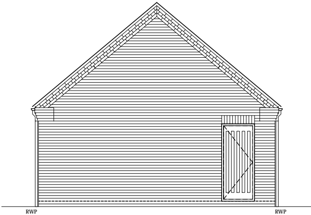
SIDE ELEVATION
