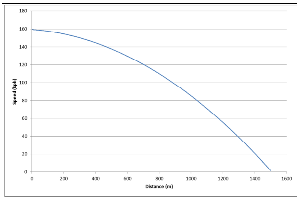
Figure 2.2 Deceleration Profile for a Class 168 DMU
