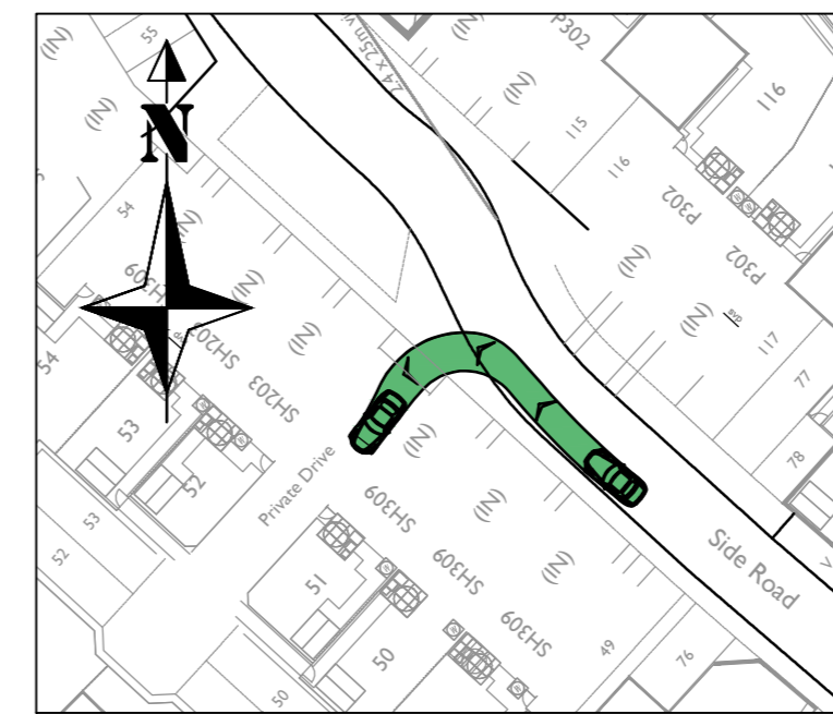
Car turning left from Road 4 into Private Driveway (Between Plots 51 & 52) Scale - 1:500
