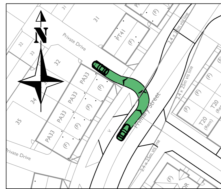
Car turning left from Road 1 into Private Driveway (Between Plots 31 & 32) Scale - 1:500
