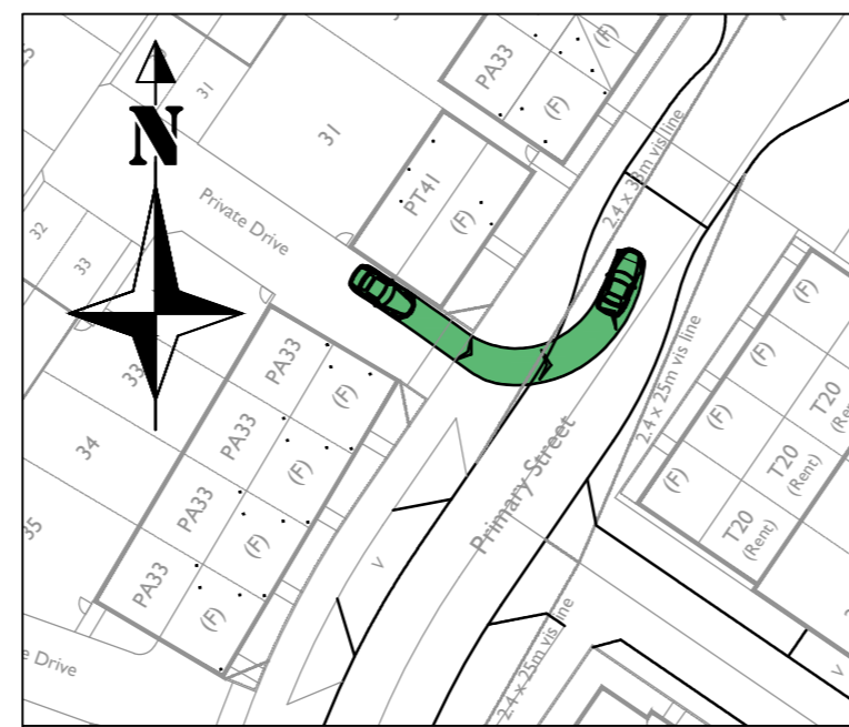
Car turning left out of Private Driveway onto Road 1 (Between Plots 31 & 32) Scale - 1:500
