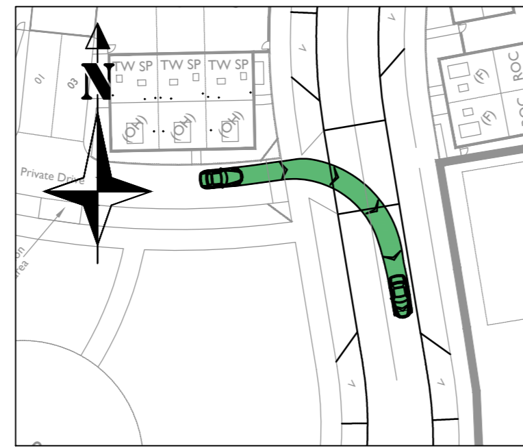
Car turning right out of Private Driveway onto Road 1 (in front of Plots 1, 2 & 3) Scale - 1:500
