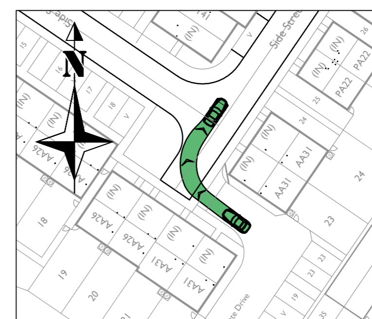
Car turning right out of Private Driveway onto Road 8 (Between Plots 21, 22 & 23) Scale - 1:500
