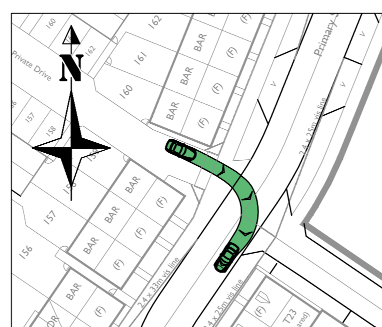
Car turning right out of Private Driveway onto Road 1 (Between Plots 157 & 158) Scale - 1:500
