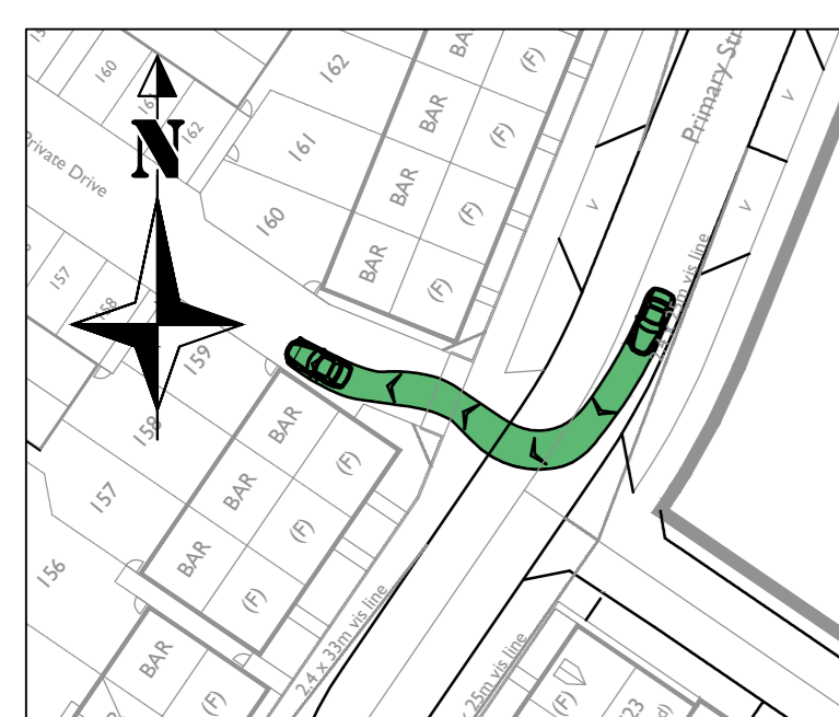
Car turning right from Road 9 into Private Driveway (Between Plots 157 & 158) Scale - 1:500
