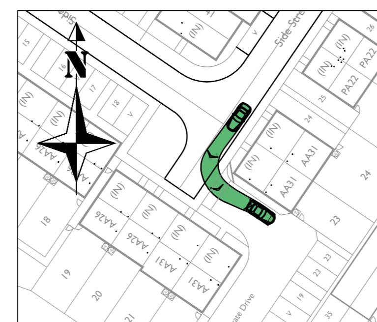
Car turning left from Road 8 into Private Driveway (Between Plots 21, 22 & 23) Scale - 1:500
