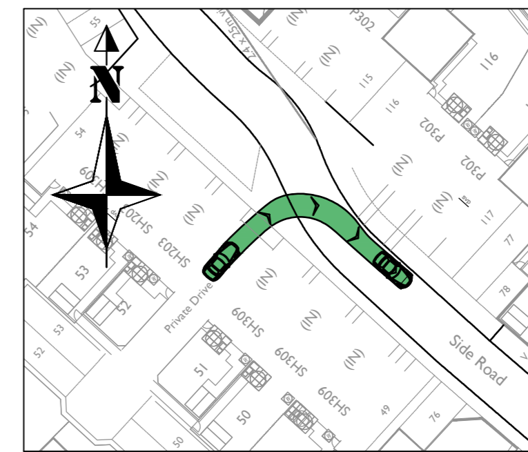
Car turning right out of Private Driveway onto Road 4 (Between Plots 51 & 52) Scale - 1:500
