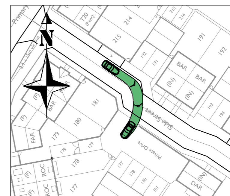
Car turning right from Road 10 into Private Driveway (Between Plots 181 & 182) Scale - 1:500
