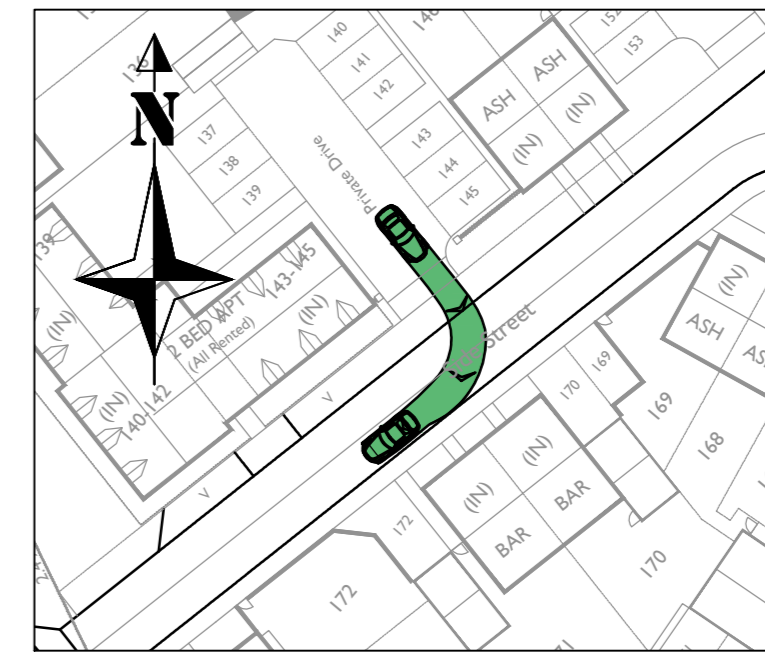
Car turning right out of Private Driveway onto Road 9 (Between Plots 143-145 & 146) Scale - 1:500
