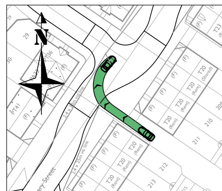
Car turning right out of Private Driveway onto Road 1 (Between Plots 211 & 212) Scale - 1:500
