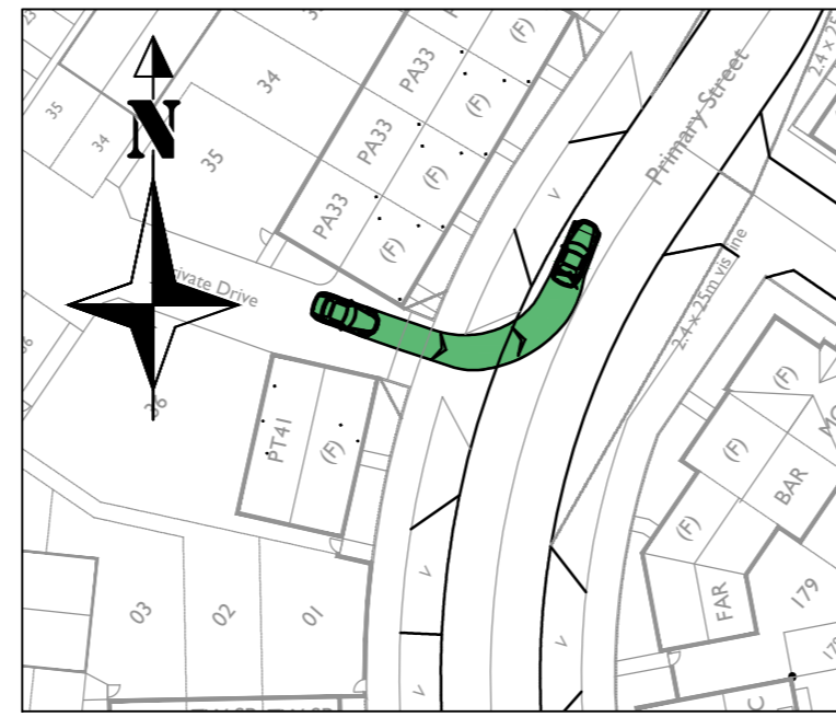
Car turning left out of Private Driveway onto Road 1 (Between Plots 35 & 36) Scale - 1:500
