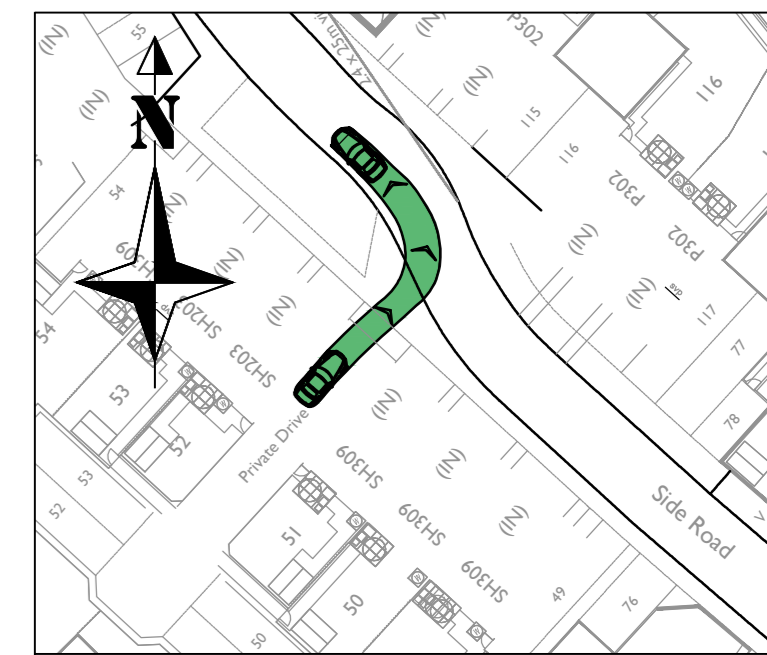
Car turning left out of Private Driveway onto Road 4 (Between Plots 51 & 52) Scale - 1:500
