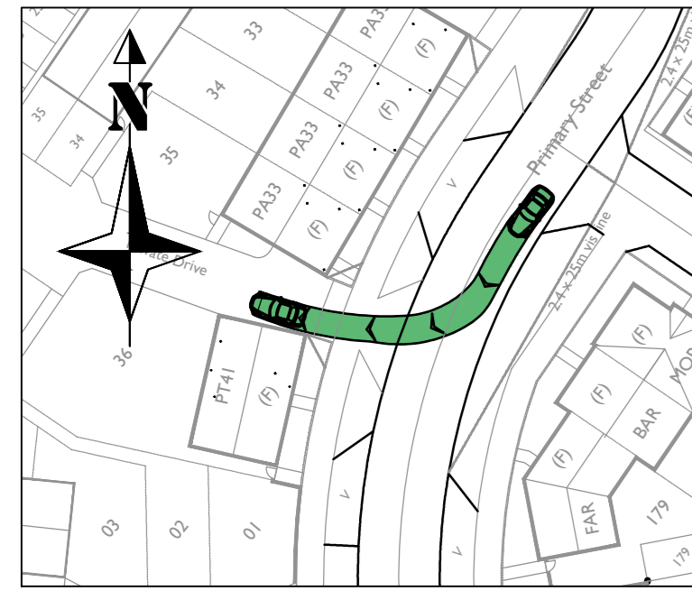
Car turning right from Road 1 into Private Driveway (Between Plots 35 & 36) Scale - 1:500
