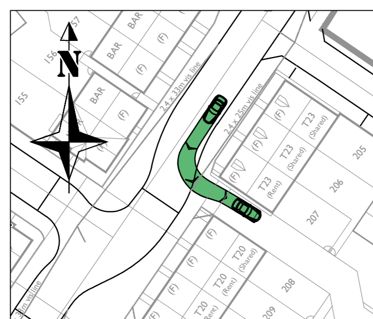
Car turning left from Road 1 into Private Driveway (Between Plots 207 & 208) Scale - 1:500
