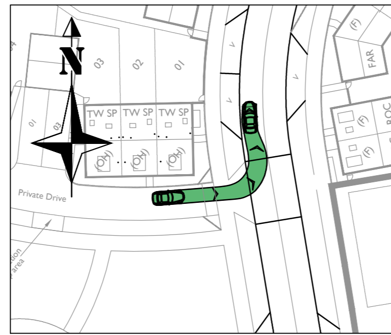
Car turning left out of Private Driveway onto Road 1 (in front of Plots 1, 2 & 3) Scale - 1:500
