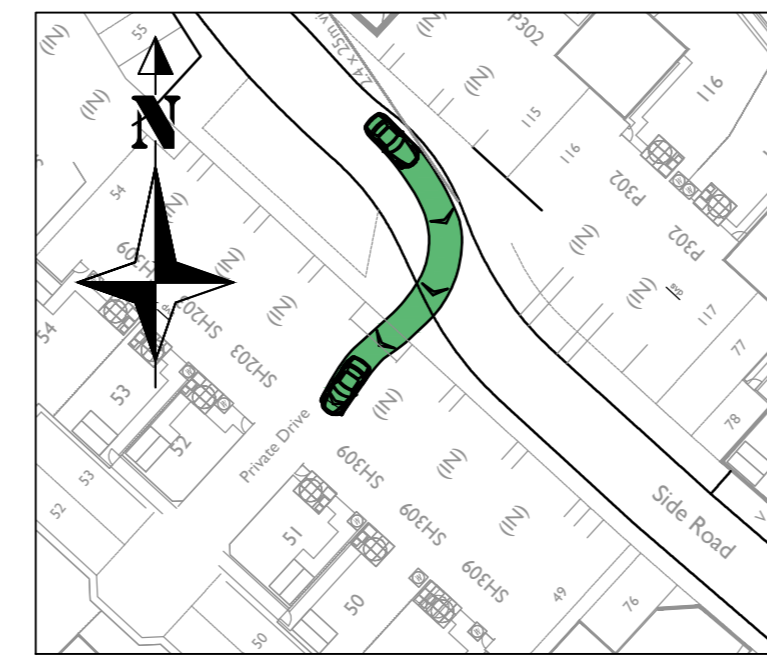
Car turning right from Road 4 into Private Driveway (Between Plots 51 & 52) Scale - 1:500
