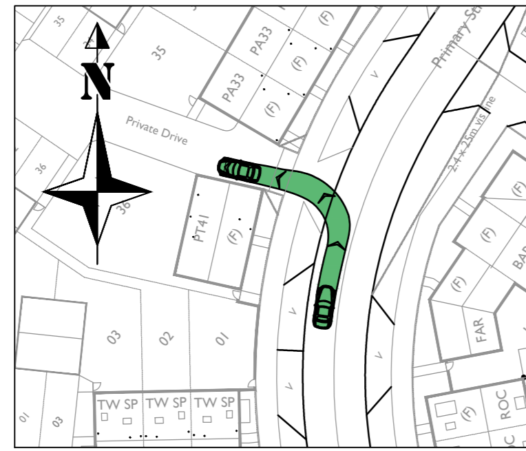
Car turning left from Road 1 into Private Driveway (Between Plots 35 & 36) Scale - 1:500
