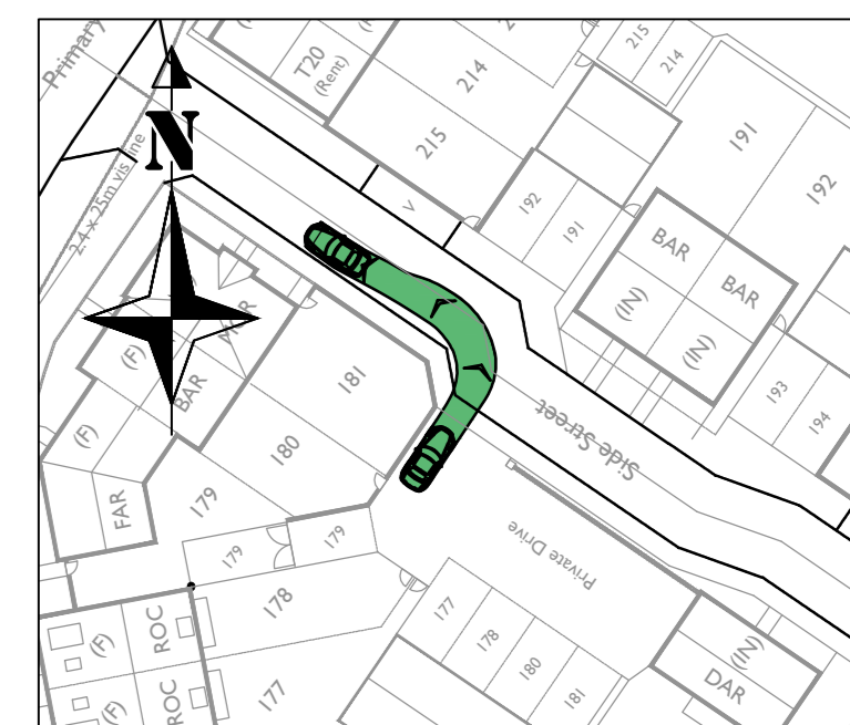
Car turning left out of Private Driveway onto Road 10 (Between Plots 181 & 182) Scale - 1:500
