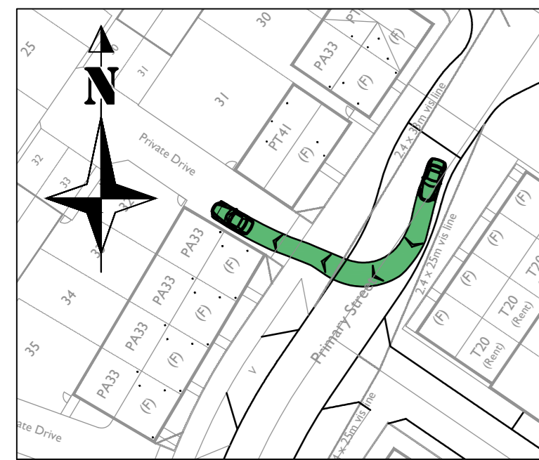
Car turning right from Road 1 into Private Driveway (Between Plots 31 & 32) Scale - 1:500
