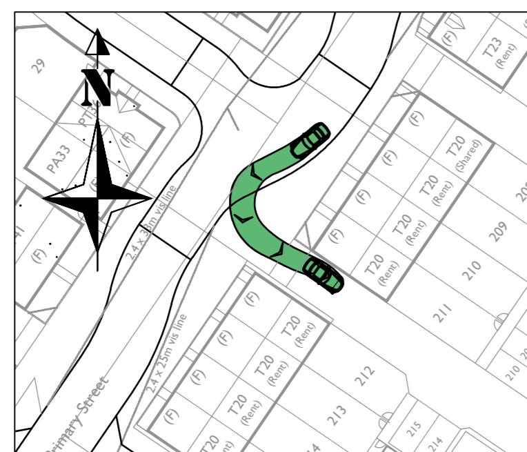
Car turning left from Road 1 into Private Driveway (Between Plots 211 & 212) Scale - 1:500
