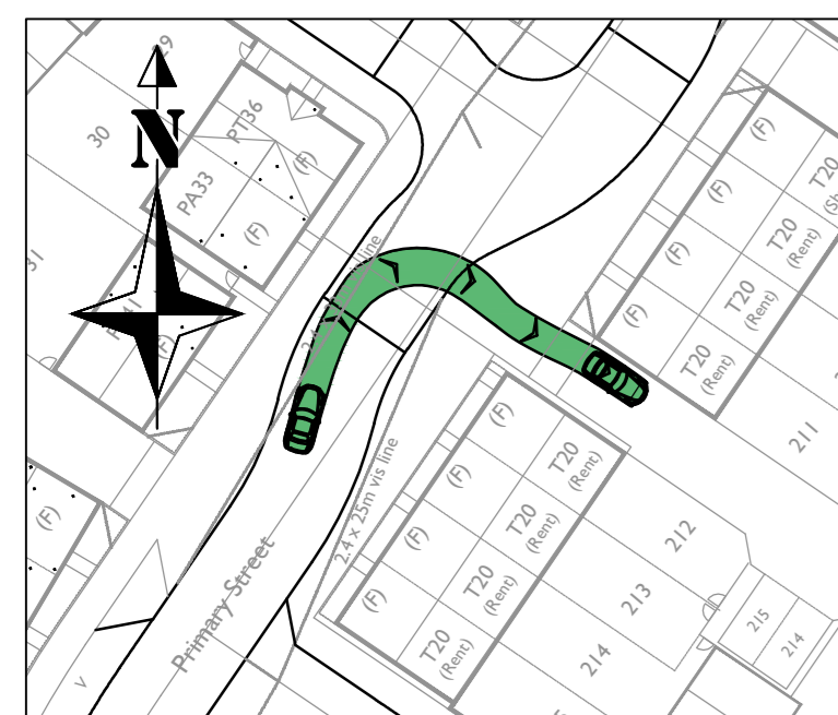
Car turning right from Road 1 into Private Driveway (Between Plots 211 & 212) Scale - 1:500
