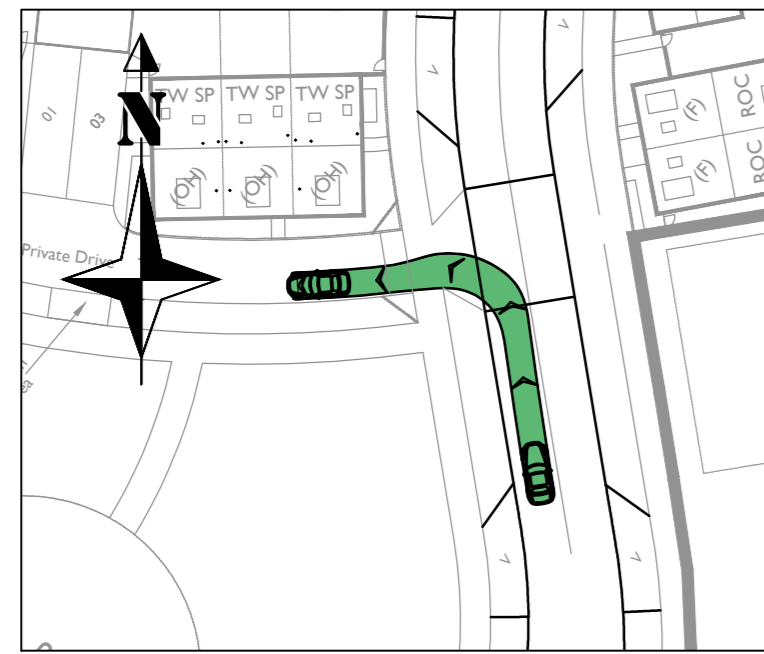
Car turning left from Road 1 into Private Driveway (in front of Plots 1, 2 & 3) Scale - 1:500
