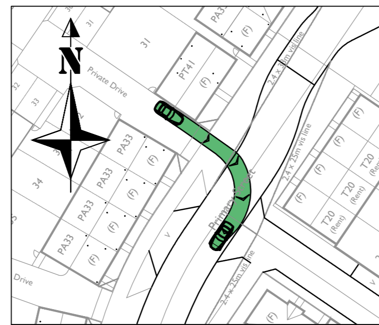
Car turning right out of Private Driveway onto Road 1 (Between Plots 31 & 32) Scale - 1:500
