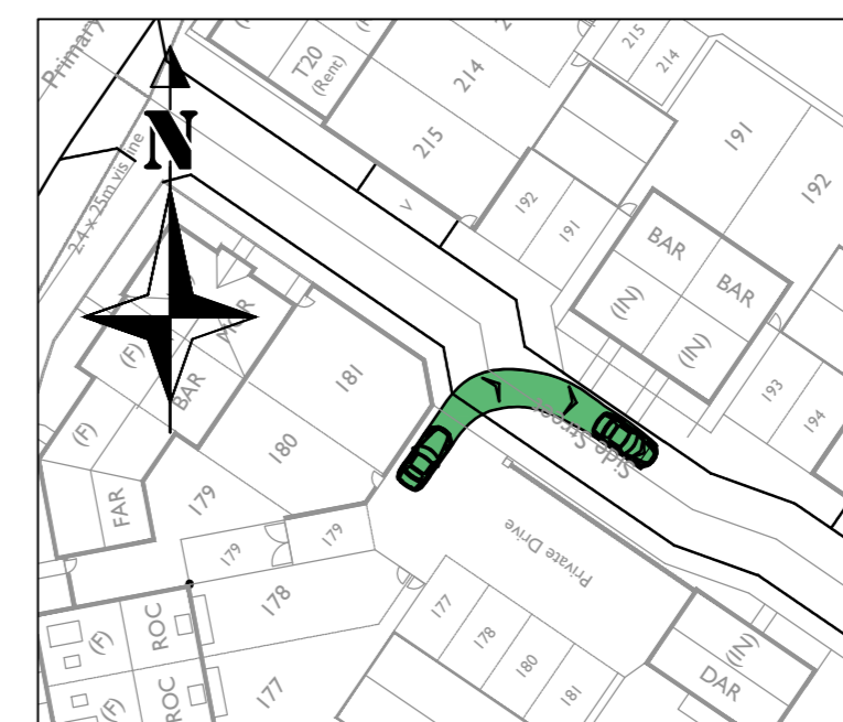
Car turning right out of Private Driveway onto Road 10 (Between Plots 181 & 182) Scale - 1:500
