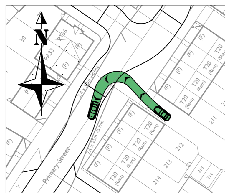
Car turning left out of Private Driveway onto Road 1 (Between Plots 211 & 212) Scale - 1:500
