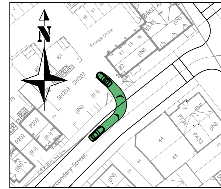
Car turning left from Road 5 into Private Driveway (Between Plots 51 & 52) Scale - 1:500
