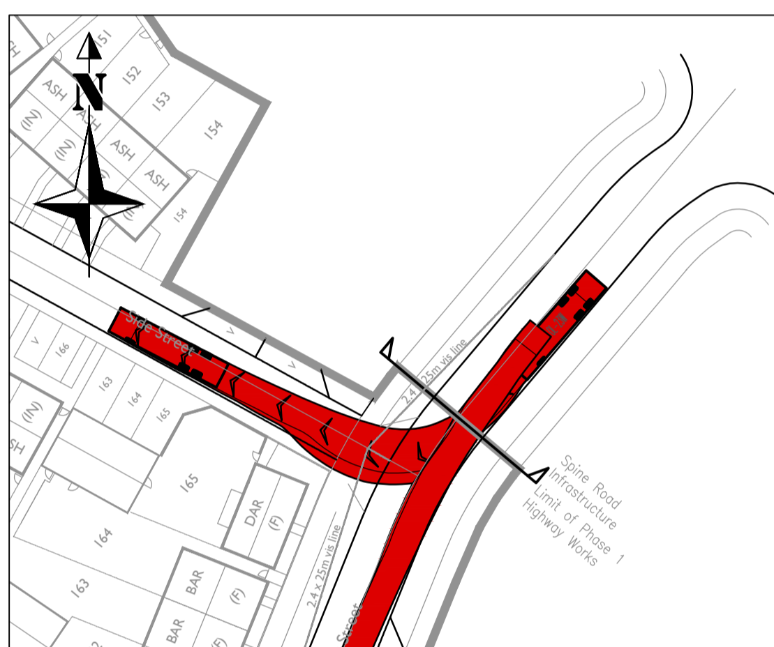
Refuse Vehicle Turning Right into junction of Roads 1 & 9
