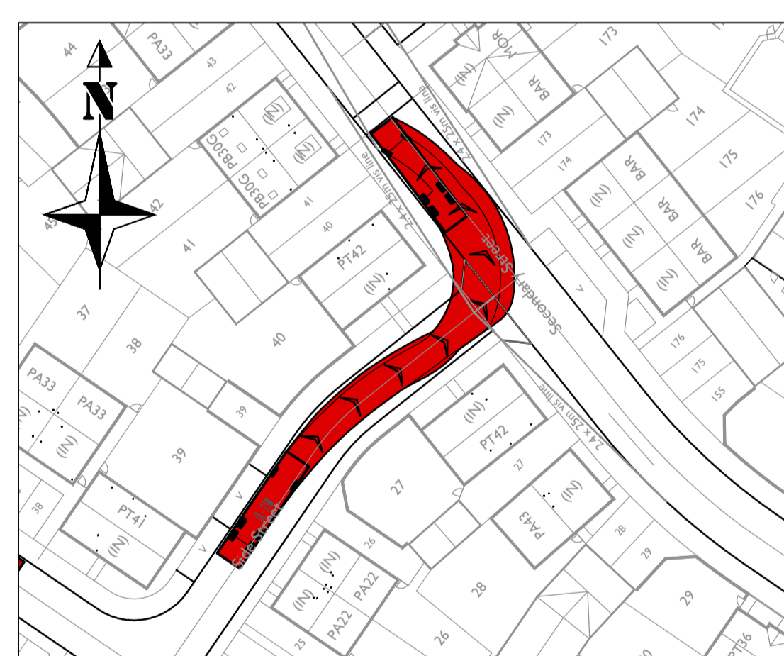
Refuse Vehicle Turning Left out of junction of Roads 8 & 2
