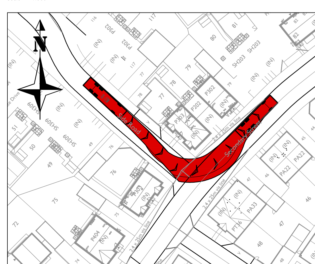
Refuse Vehicle Turning Left out of junction of Roads 4 & 6
