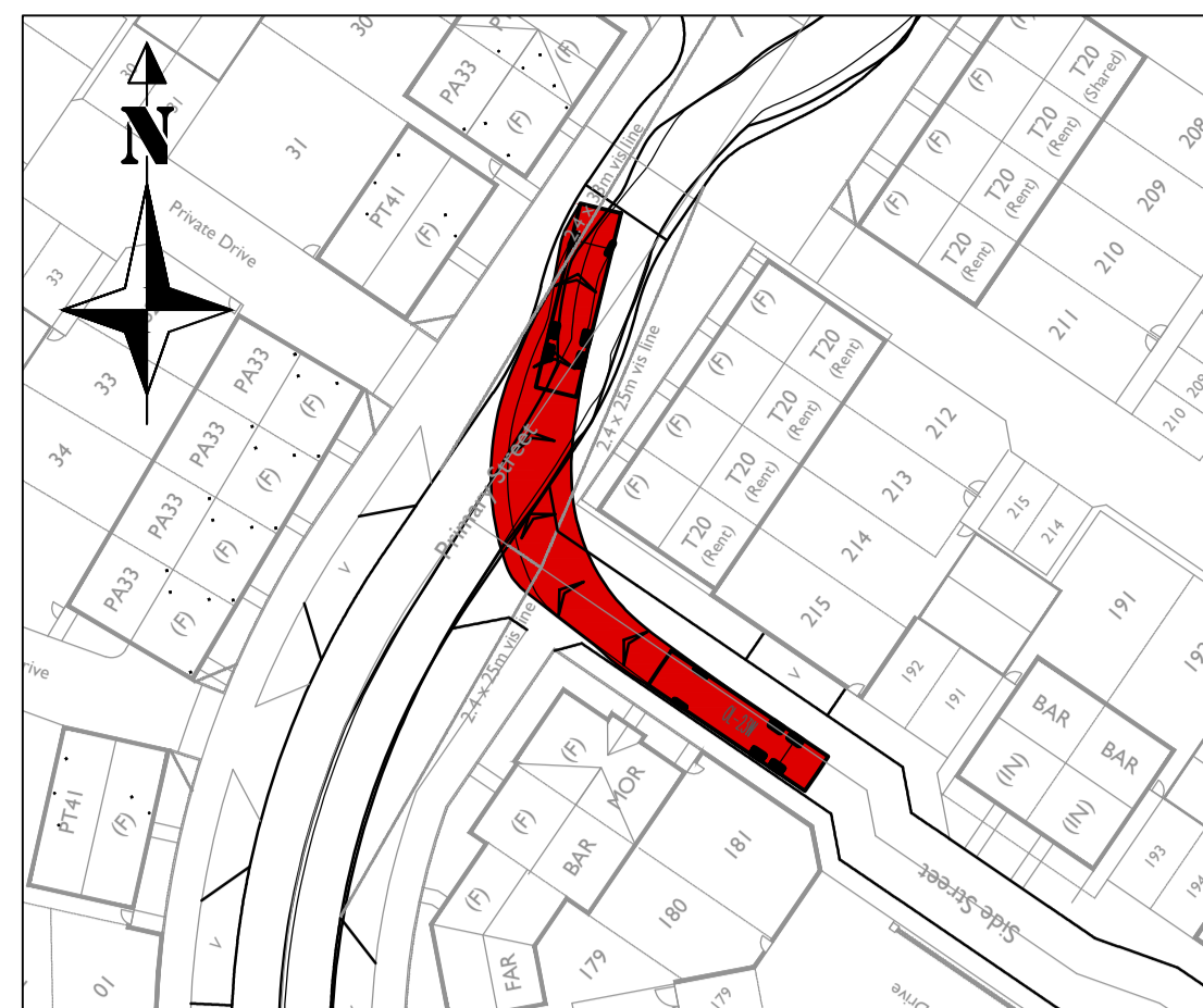
Refuse Vehicle Turning Right out of junction of Roads 10 & 1 (West)
