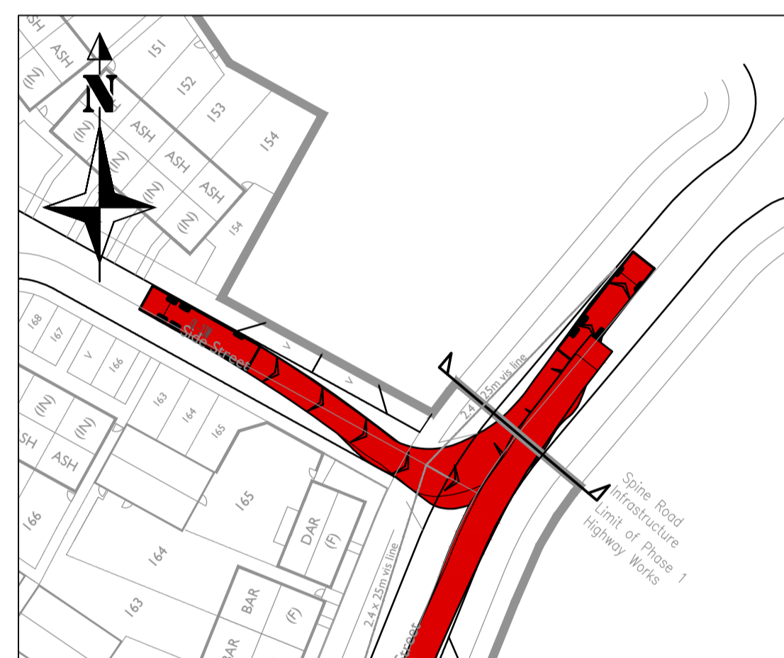
Refuse Vehicle Turning Left out of junction of Roads 9 & 1
