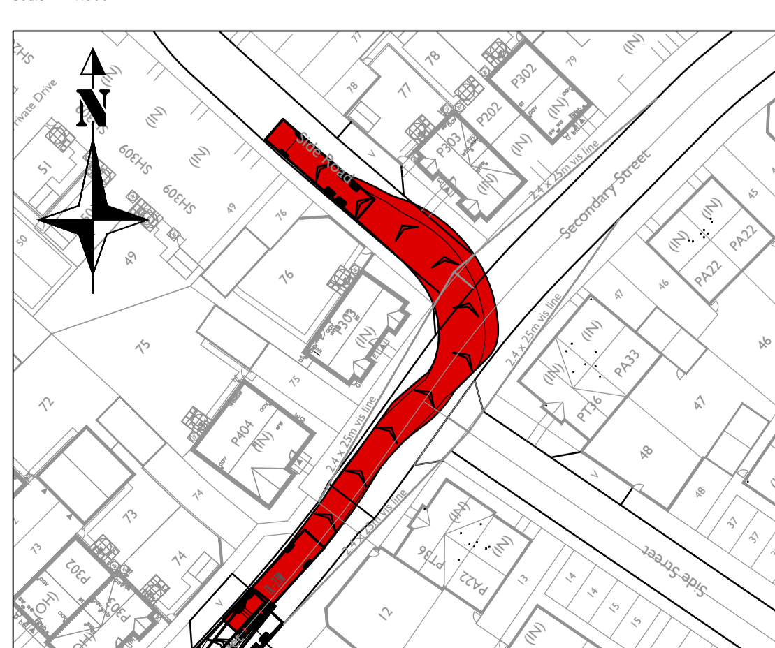
Refuse Vehicle Turning Left into junction of Roads 6 & 4
