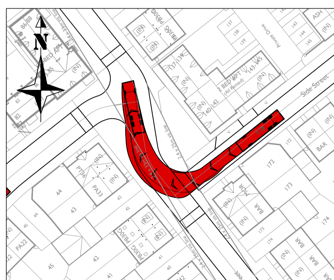
Refuse Vehicle Turning Right out of junction of Roads 9 & 2
