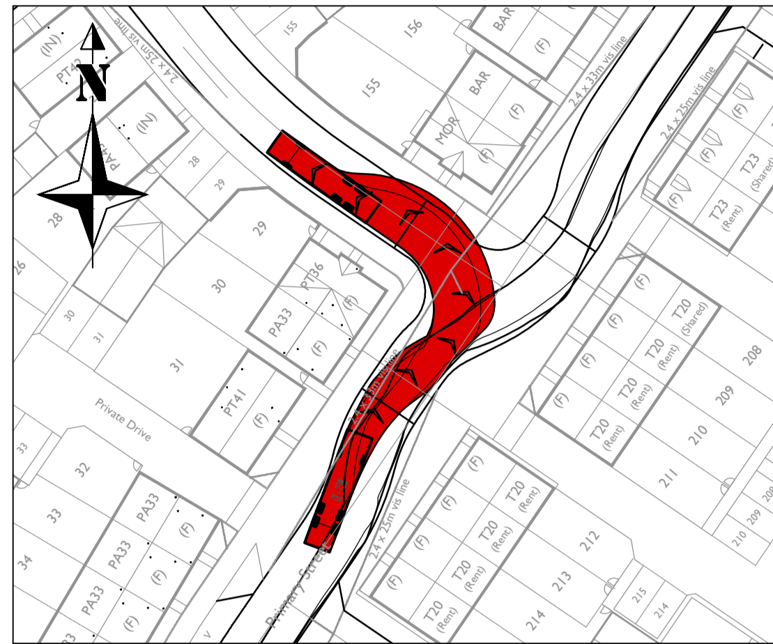
Refuse Vehicle Turning Left into junction of Roads 1 & 2
