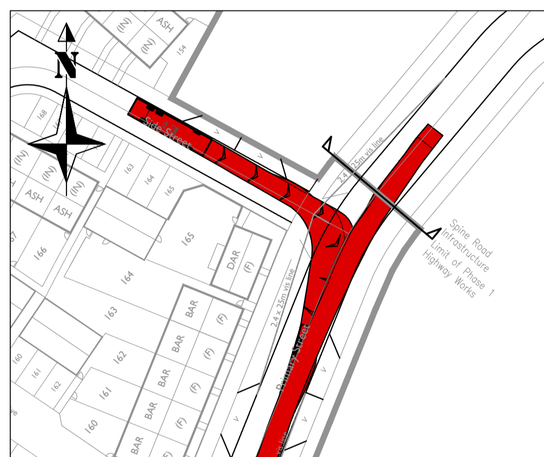
Refuse Vehicle Turning Right out of junction of Roads 9 & 1
