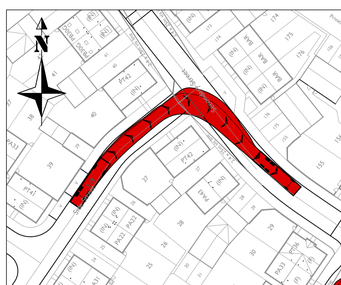
Refuse Vehicle Turning Right out of junction of Roads 8 & 2
