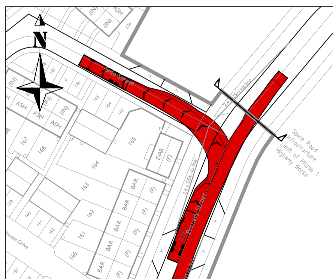
Refuse Vehicle Turning Left into junction of Roads 1 & 9
