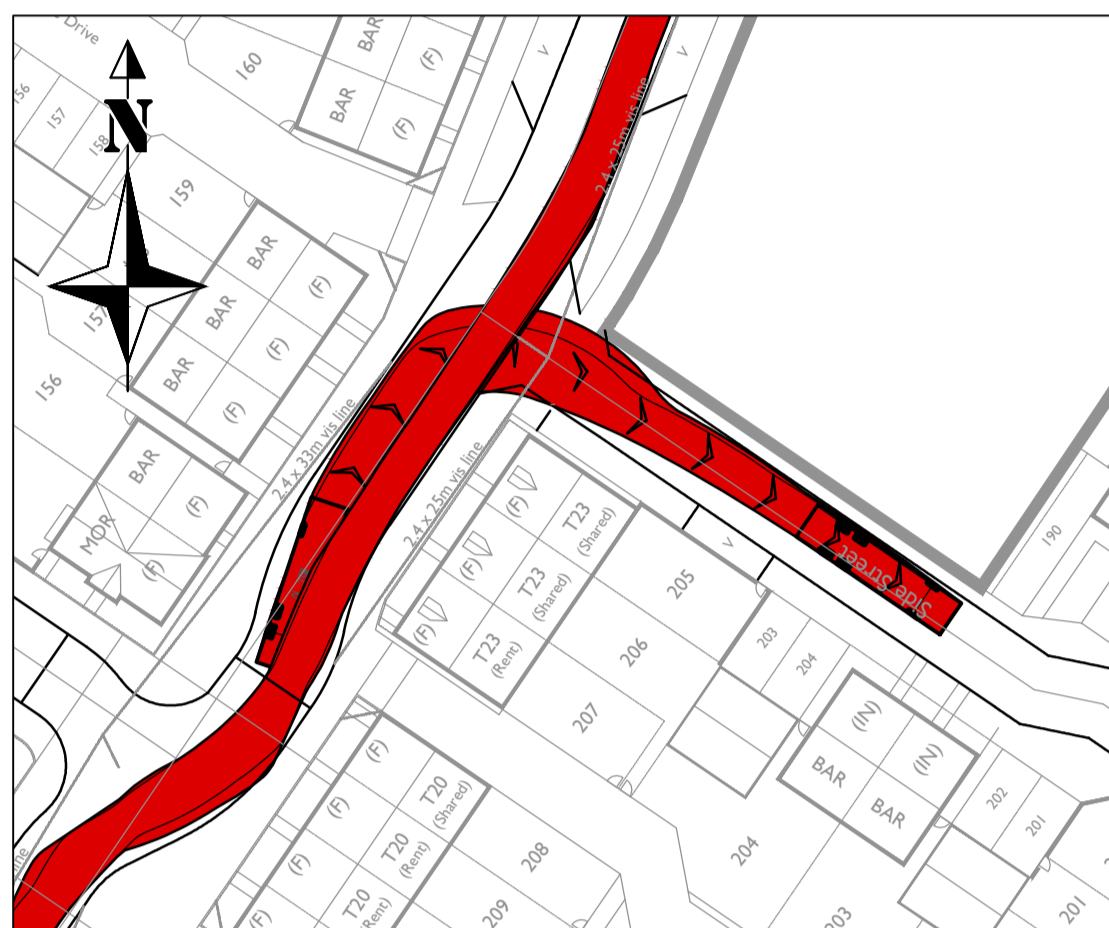
Refuse Vehicle Turning Right into junction of Roads 1 & 2 (East)
