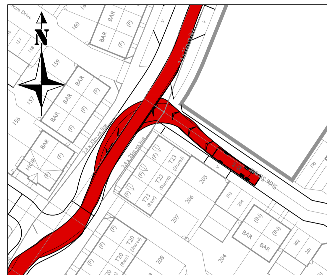
Refuse Vehicle Turning Left out of junction of Roads 2 & 1 (East)
