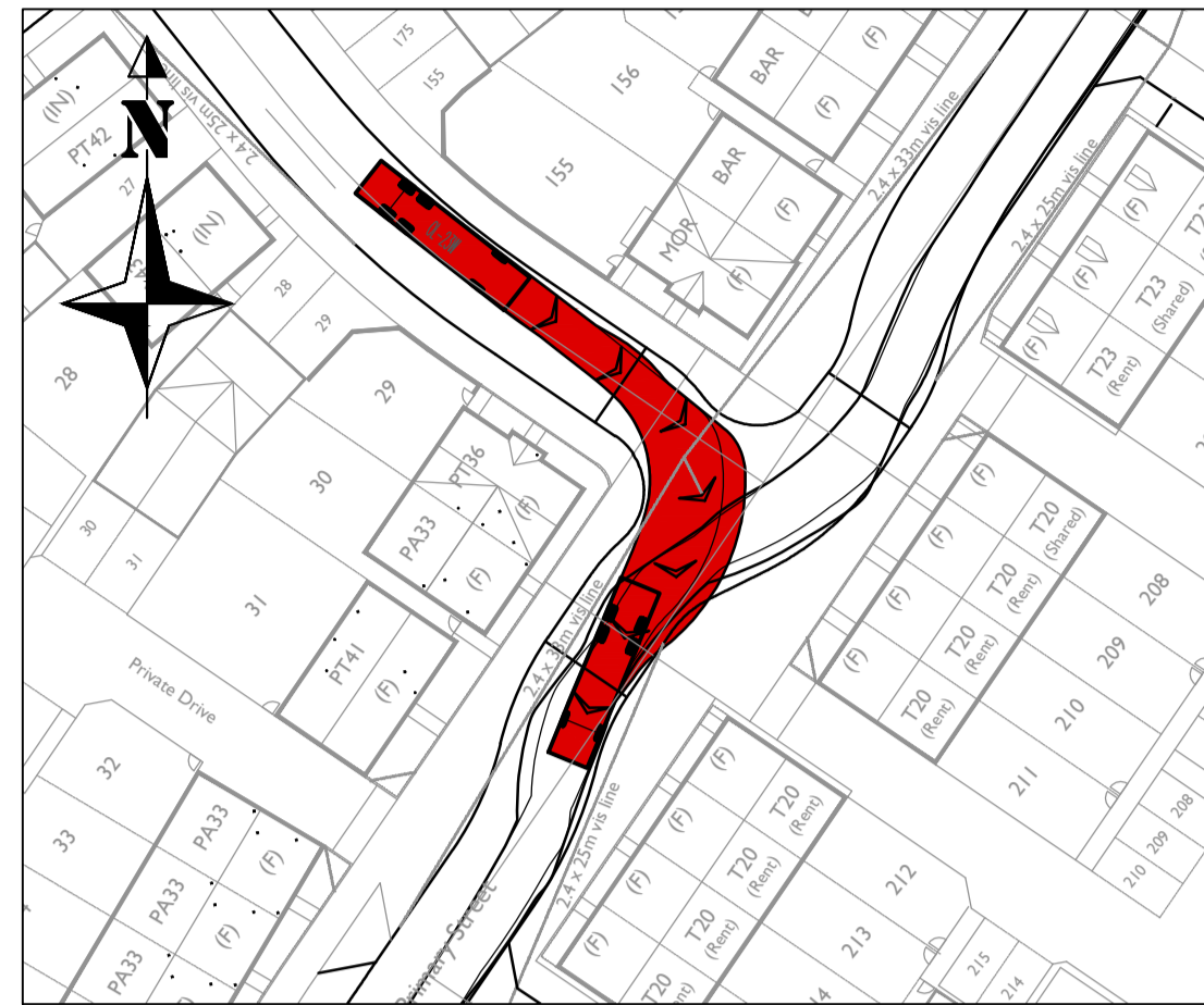
Refuse Vehicle Turning Right out of junction of Roads 2 & 1
