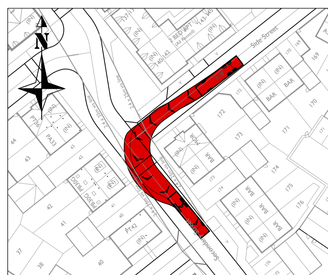
Refuse Vehicle Turning Left out of junction of Roads 9 & 2
