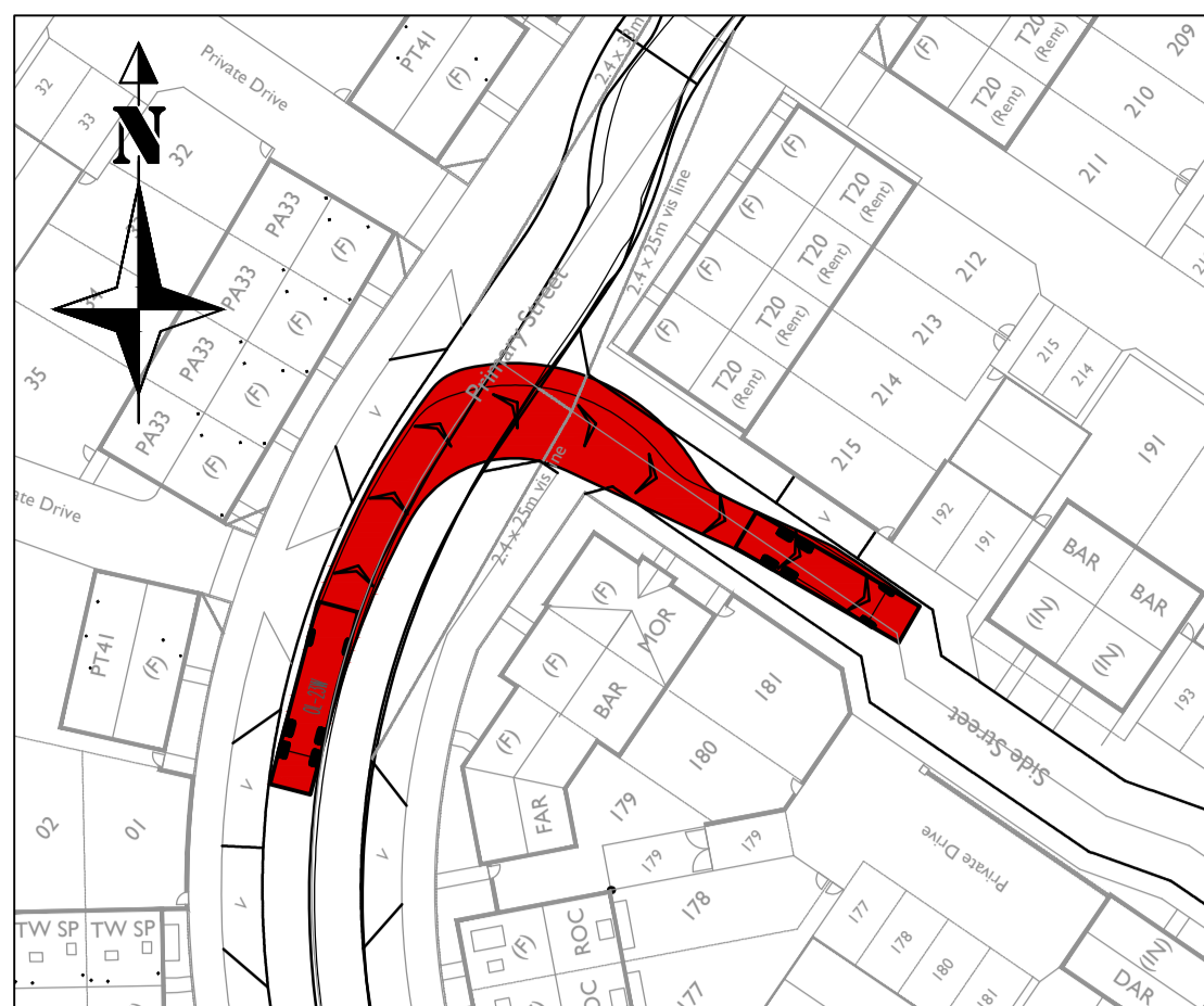
Refuse Vehicle Turning Right into junction of Roads 1 & 10 (West)
