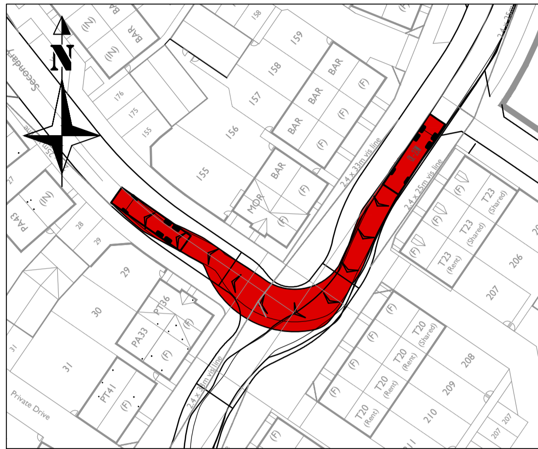
Refuse Vehicle Turning Right into junction of Roads 1 & 2
