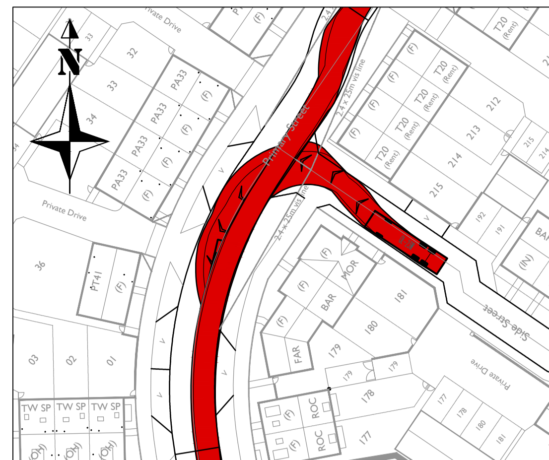
Refuse Vehicle Turning Left out of junction of Roads 10 & 1 (West)
