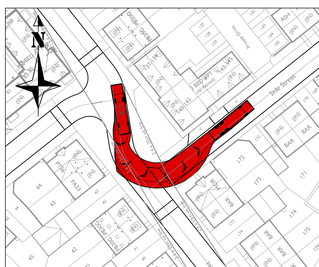
Refuse Vehicle Turning Left into junction of Roads 2 & 9
