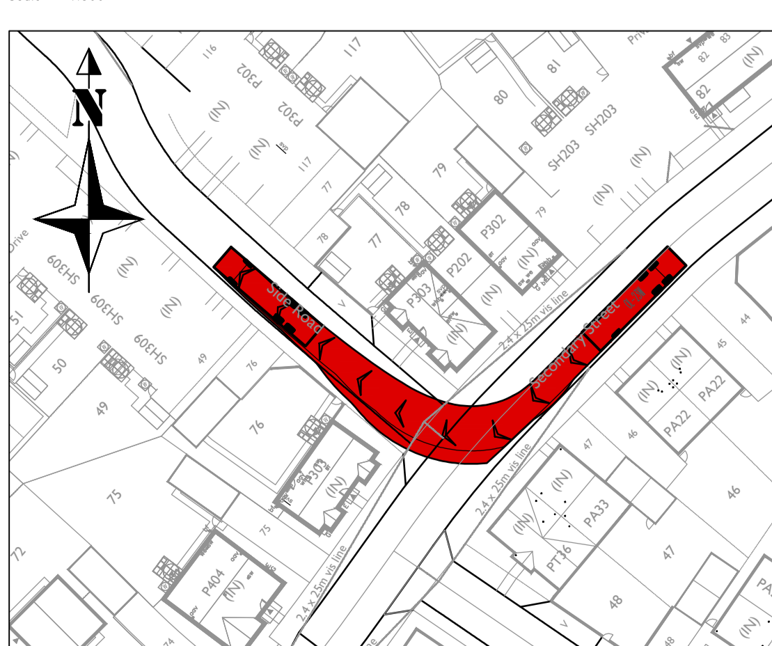
Refuse Vehicle Turning Right into junction of Roads 6 & 4
