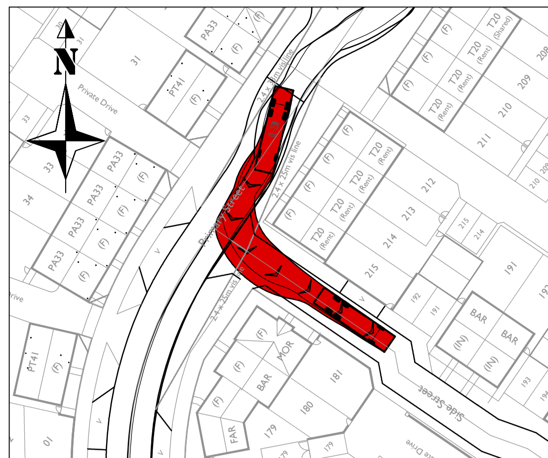
Refuse Vehicle Turning Left into junction of Roads 1 & 10 (West)
