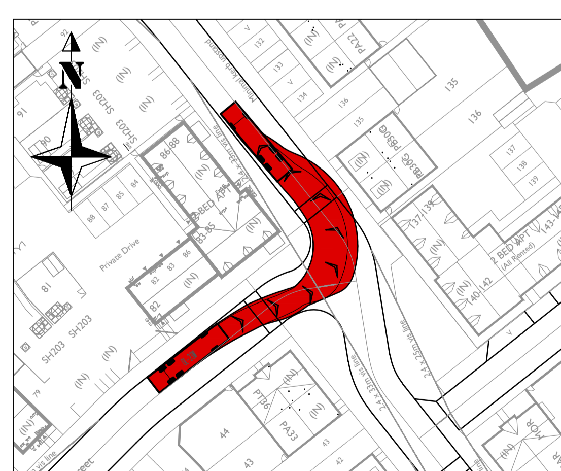
Refuse Vehicle Turning Left out of junction of Roads 6 & 2
