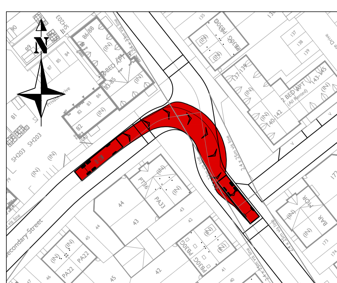
Refuse Vehicle Turning Right out of junction of Roads 6 & 2
