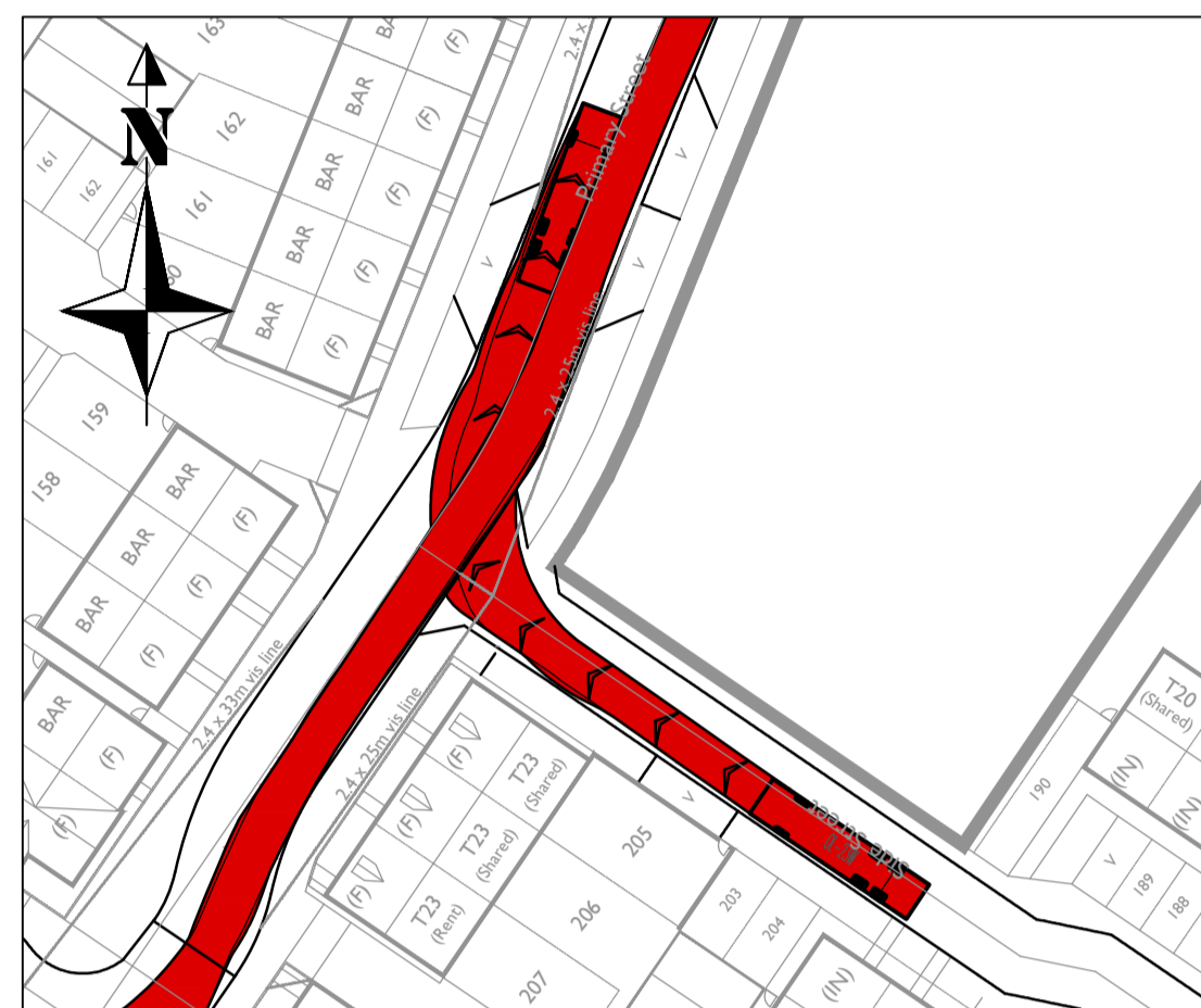
Refuse Vehicle Turning Right out of junction of Roads 2 & 1 (East)
