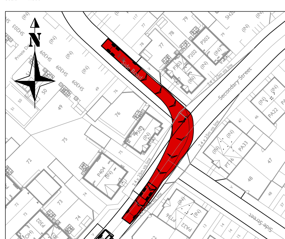
Refuse Vehicle Turning Right out of junction of Roads 4 & 6
