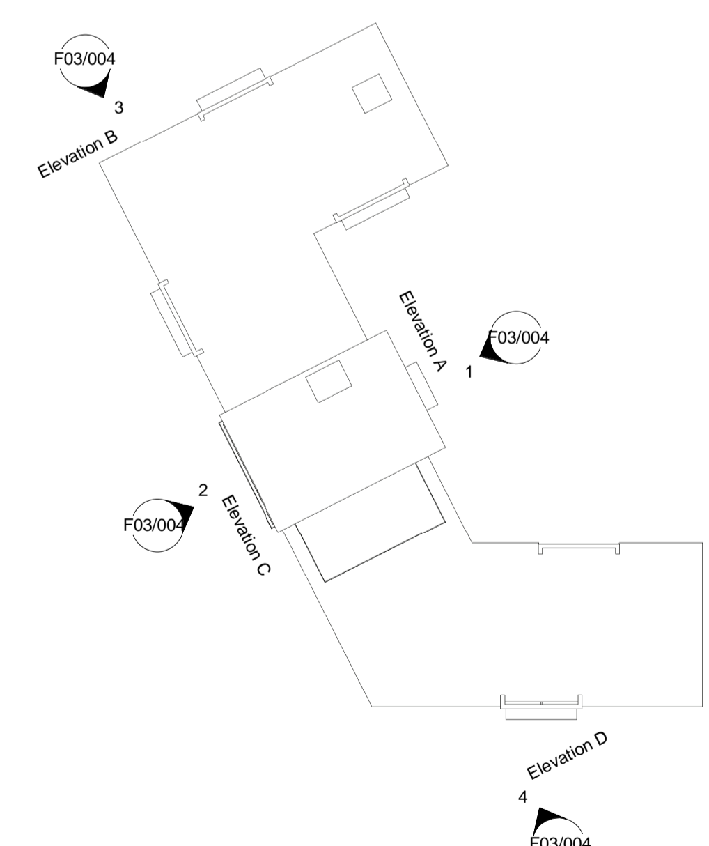
5 Elevation Key 1:500
