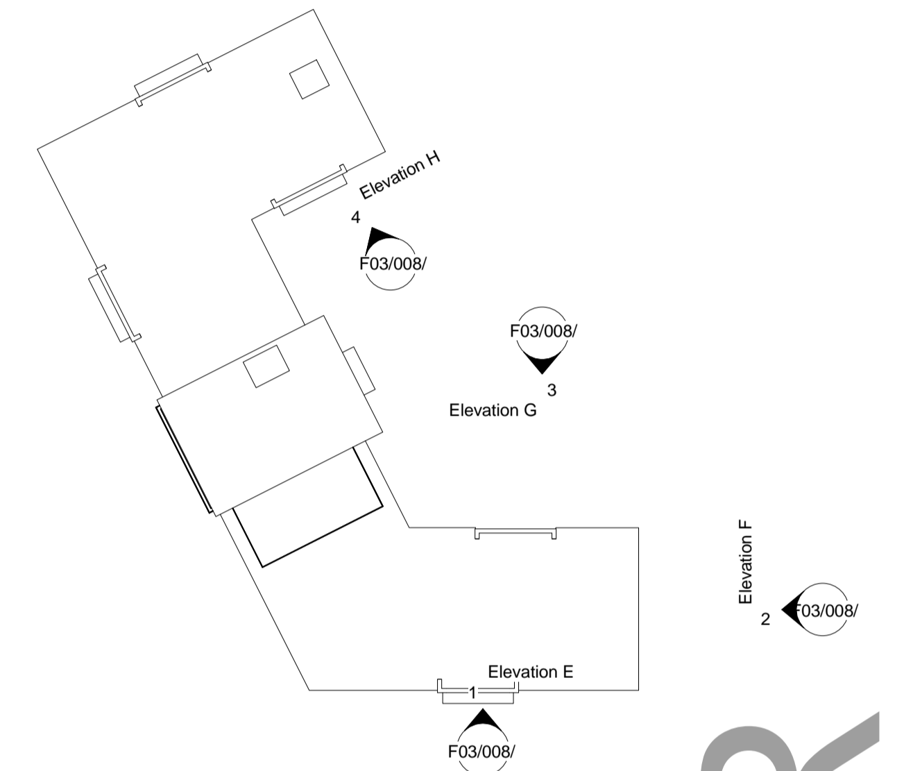
5 ELEVATION KEY 1:500
