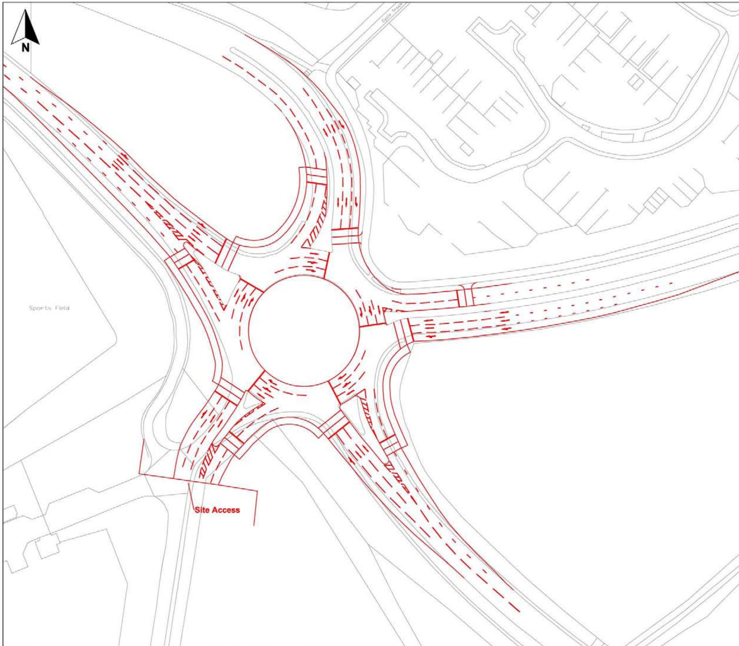
Figure 11.3 A41/Gravenhill Road/B4100 - Mitigation Scheme (signal)
