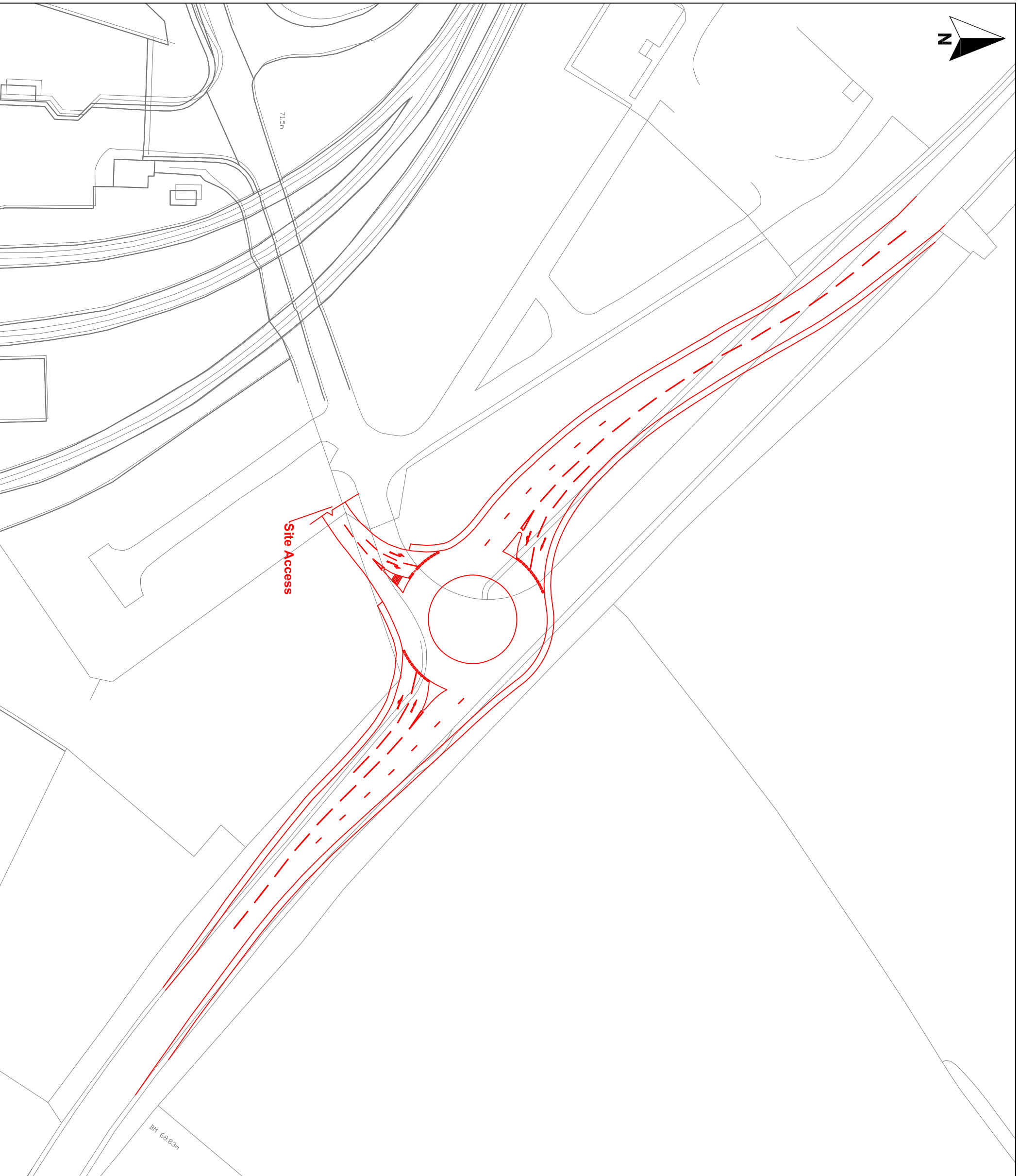
Figure 14 A41/Pioneer Road - Mitigation Scheme
