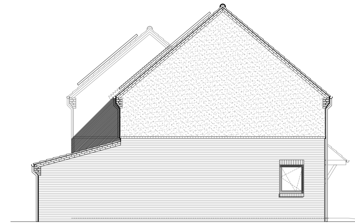
SIDE ELEVATION 2 - PLOTS 314 & 330
