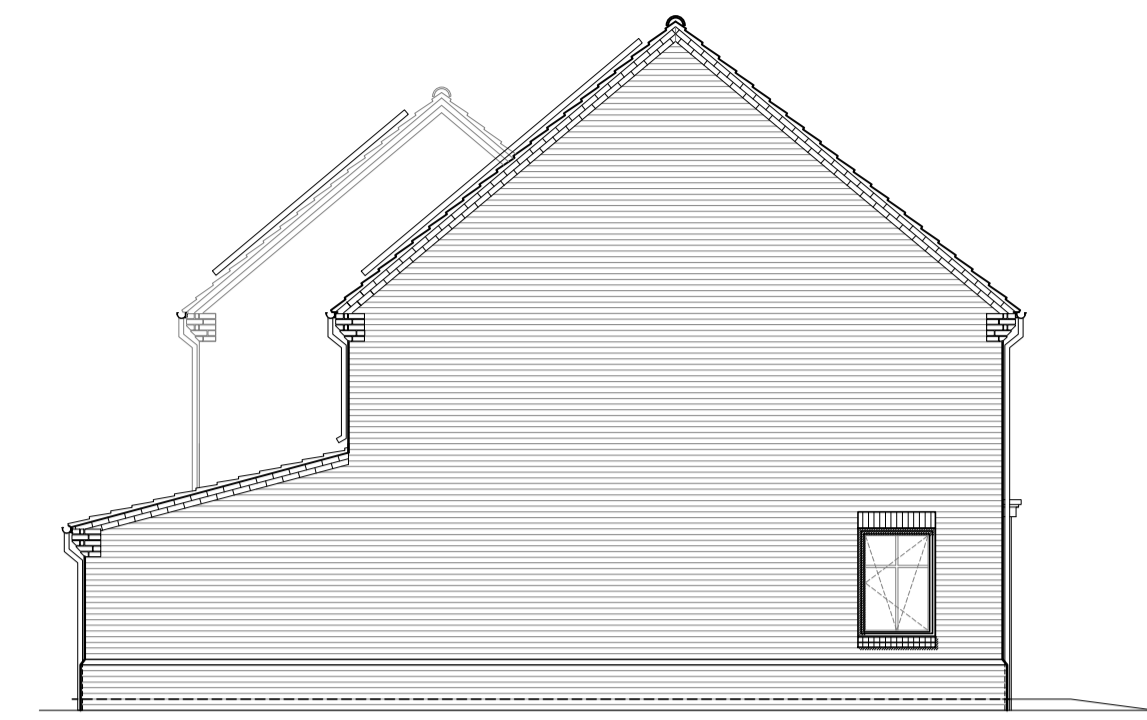
SIDE ELEVATION 2 - PLOTS 309 & 310
