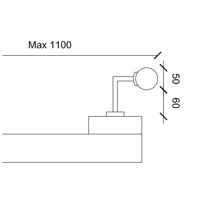
DDA handrail fixing detail 1:5 @ A1
