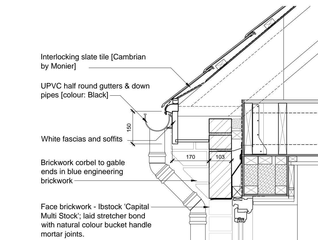
DETAIL 1 - Eaves
