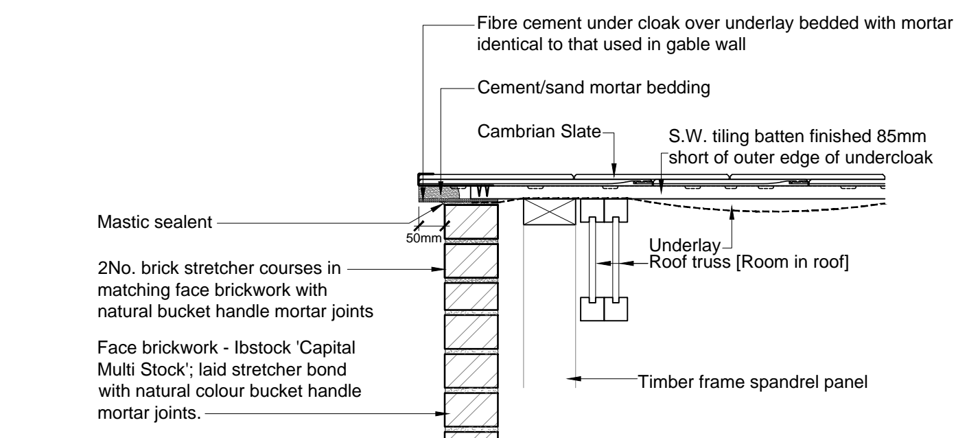
DETAIL 6 - Mortar Bedded Verge - Type 5 dwellings - (Brickwork)
