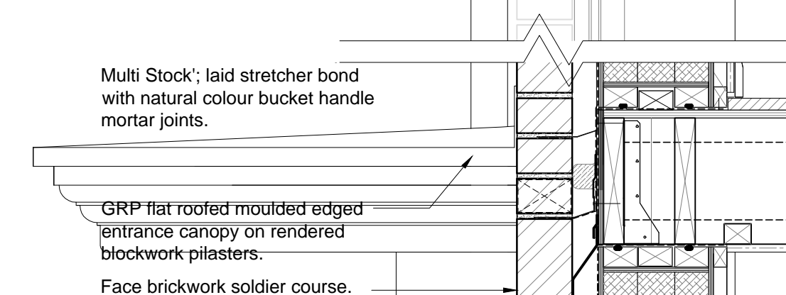
DETAIL 2 - Face Brickwork Window / Door Heads
