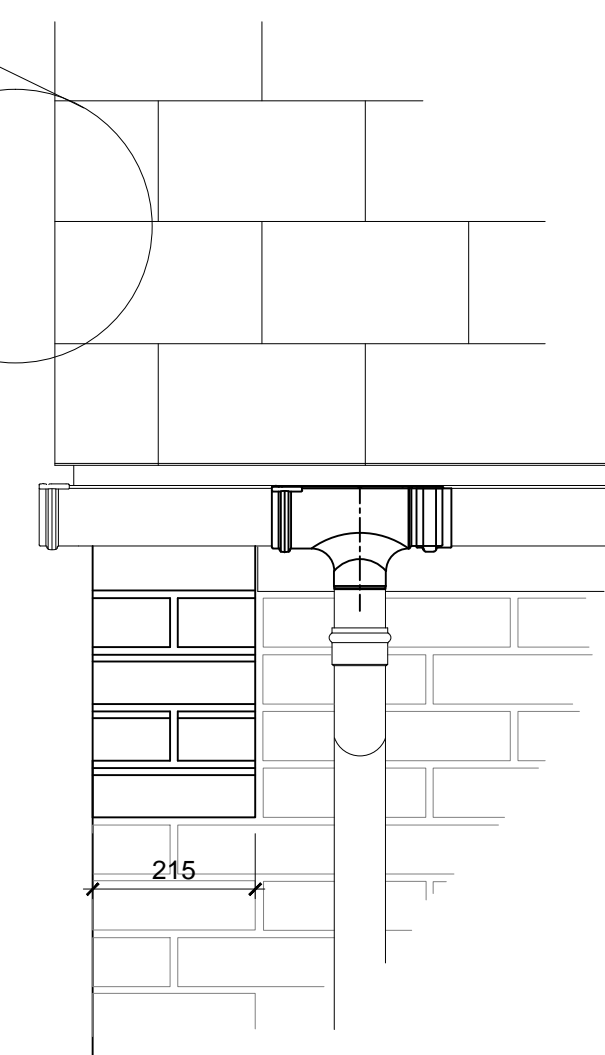
DETAIL 5 - Corbel detail Type 5 dwellings (Brickwork) Scale 1:10
