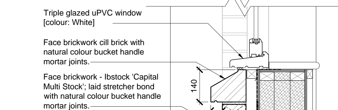
DETAIL 3 - Face brickwork soldier course windowcill
