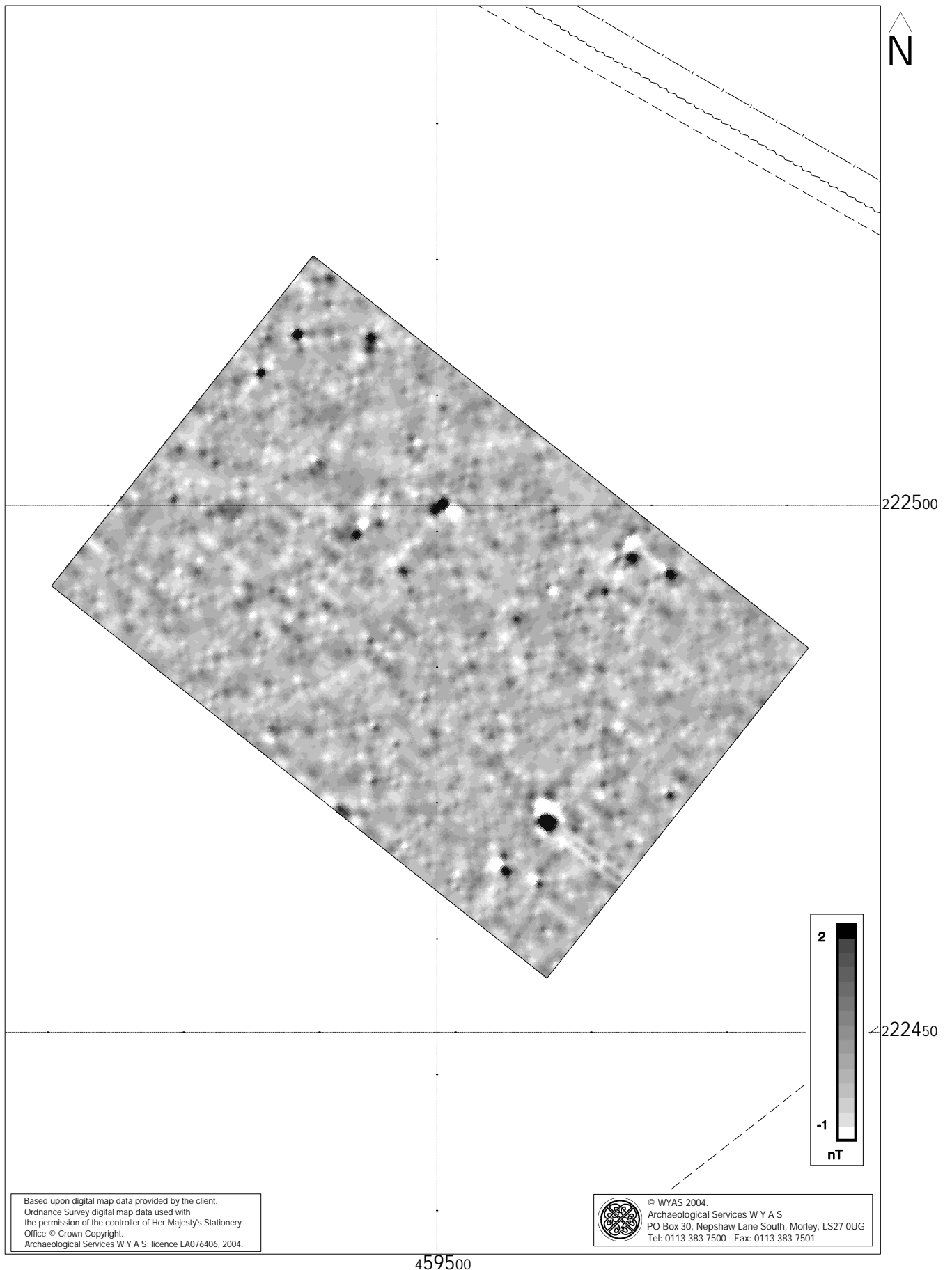
Fig. 3. Greyscale plot of gradiometer data; Block 1
