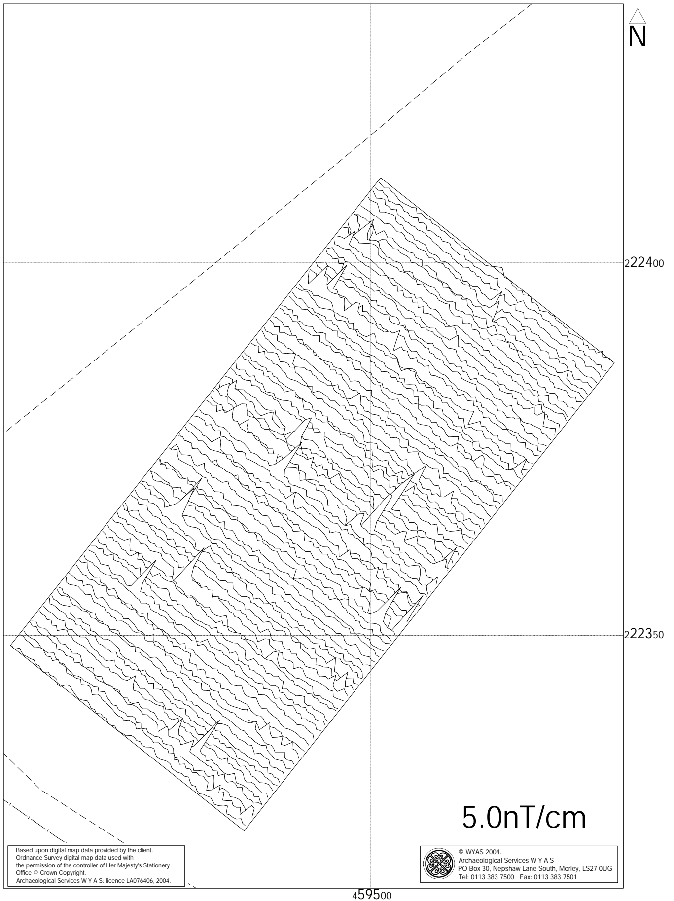
Fig. 14. XY trace plot of gradiometer data; Block 4
