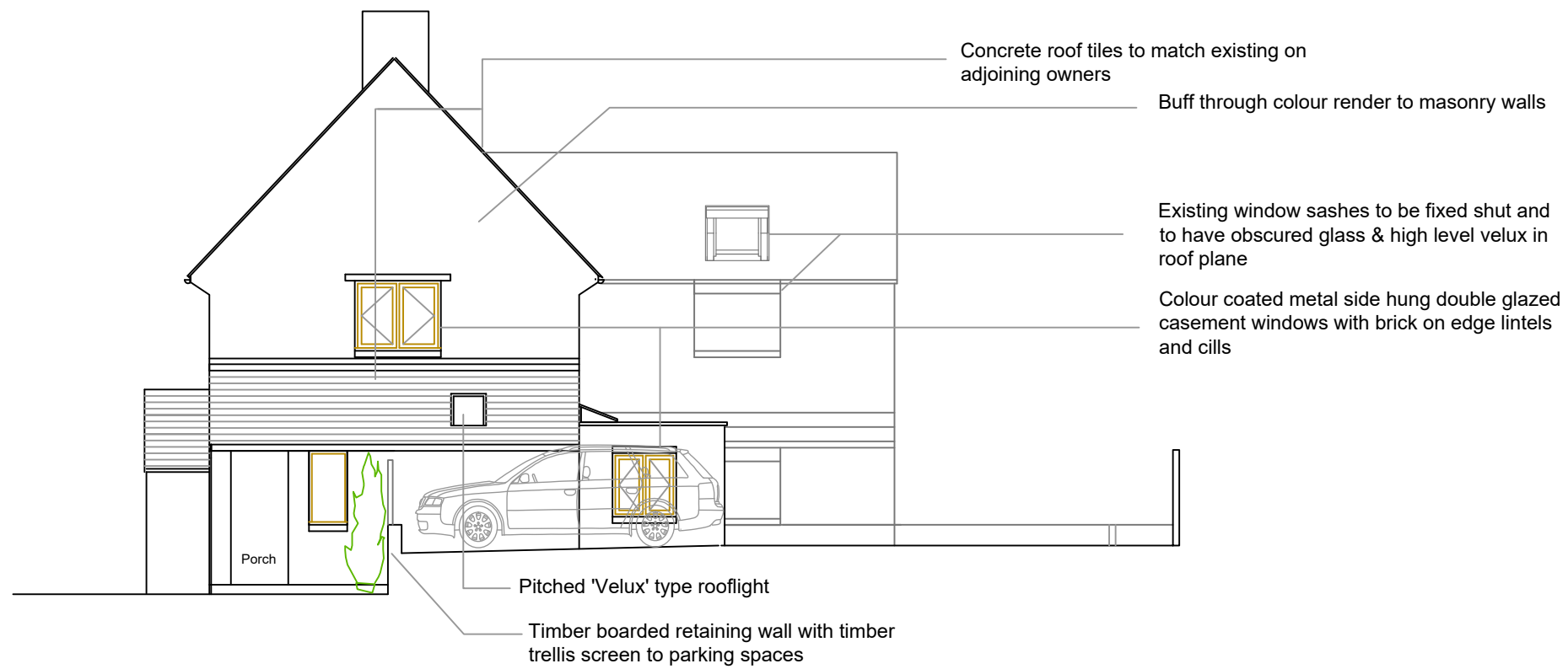
NORTH EAST SECTIONAL ELEVATION X-X
