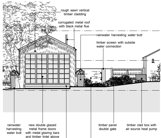
Proposed Garden Room - South East Elevation
