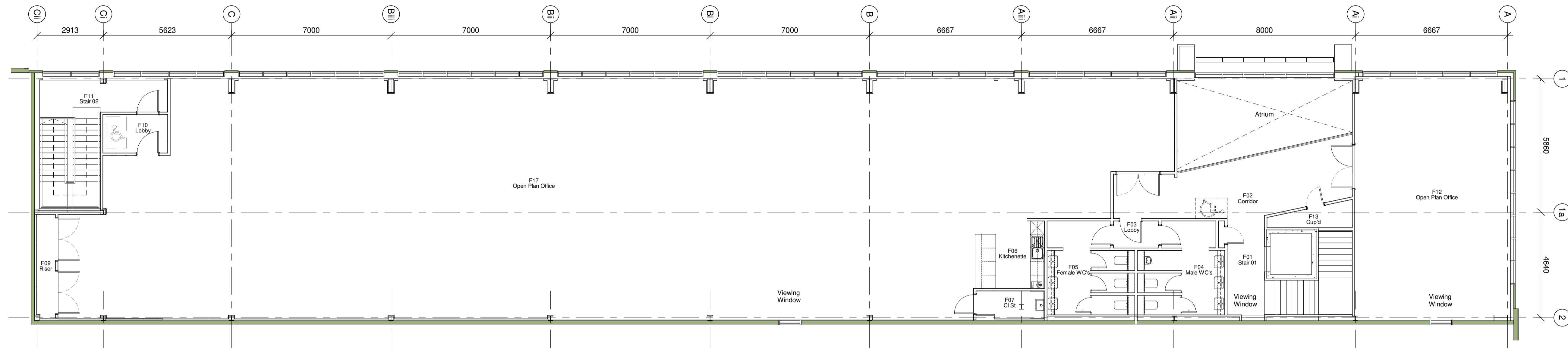
2 GA Level 01 Main Office Plan 1:100
