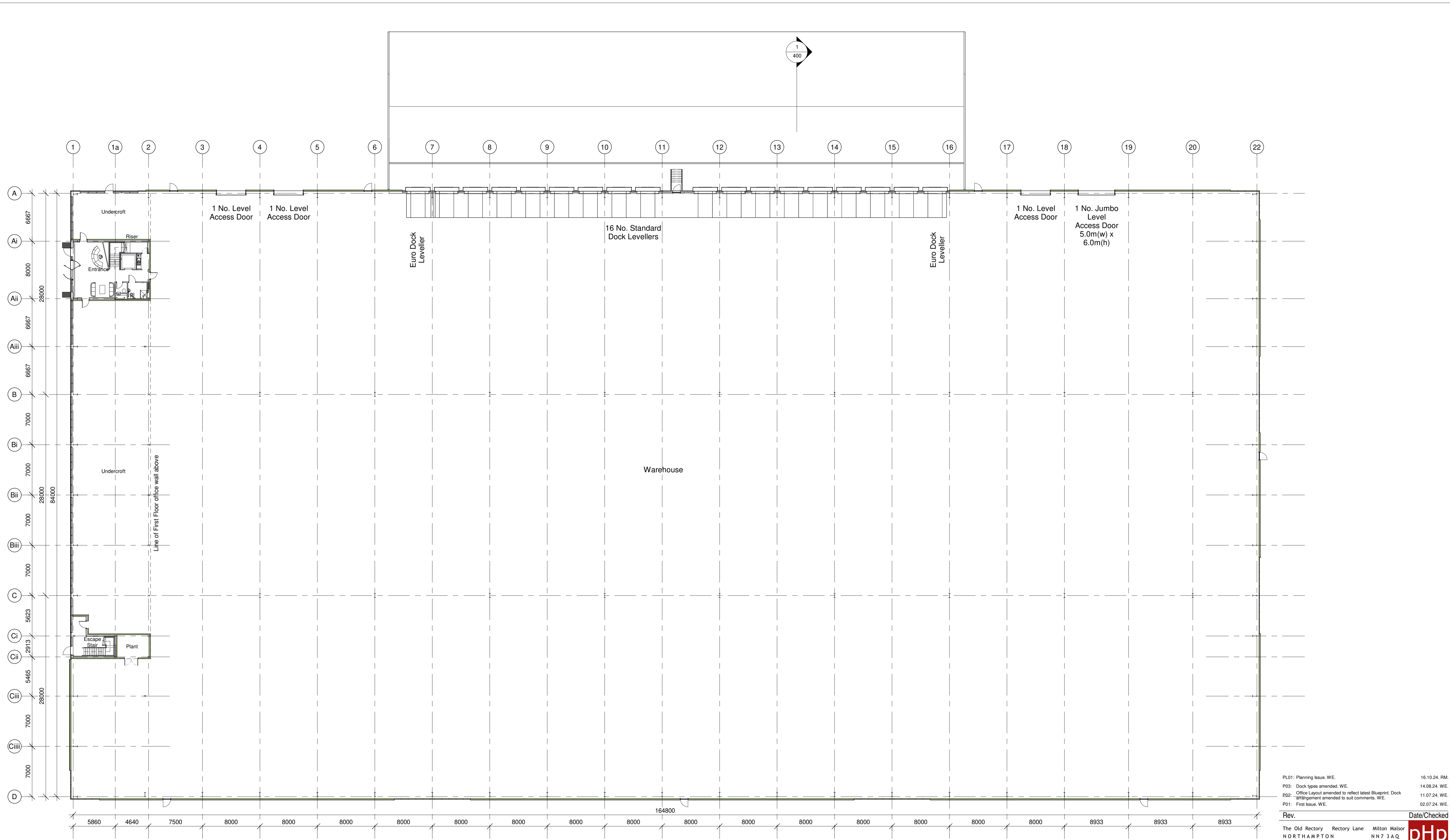
1 GA Level 00 Plan 1 : 250
