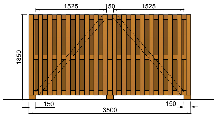
SIDE ELEVATION OF BIN STORE
