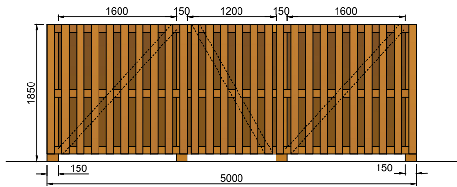
FRONT ELEVATION OF BIN STORE
