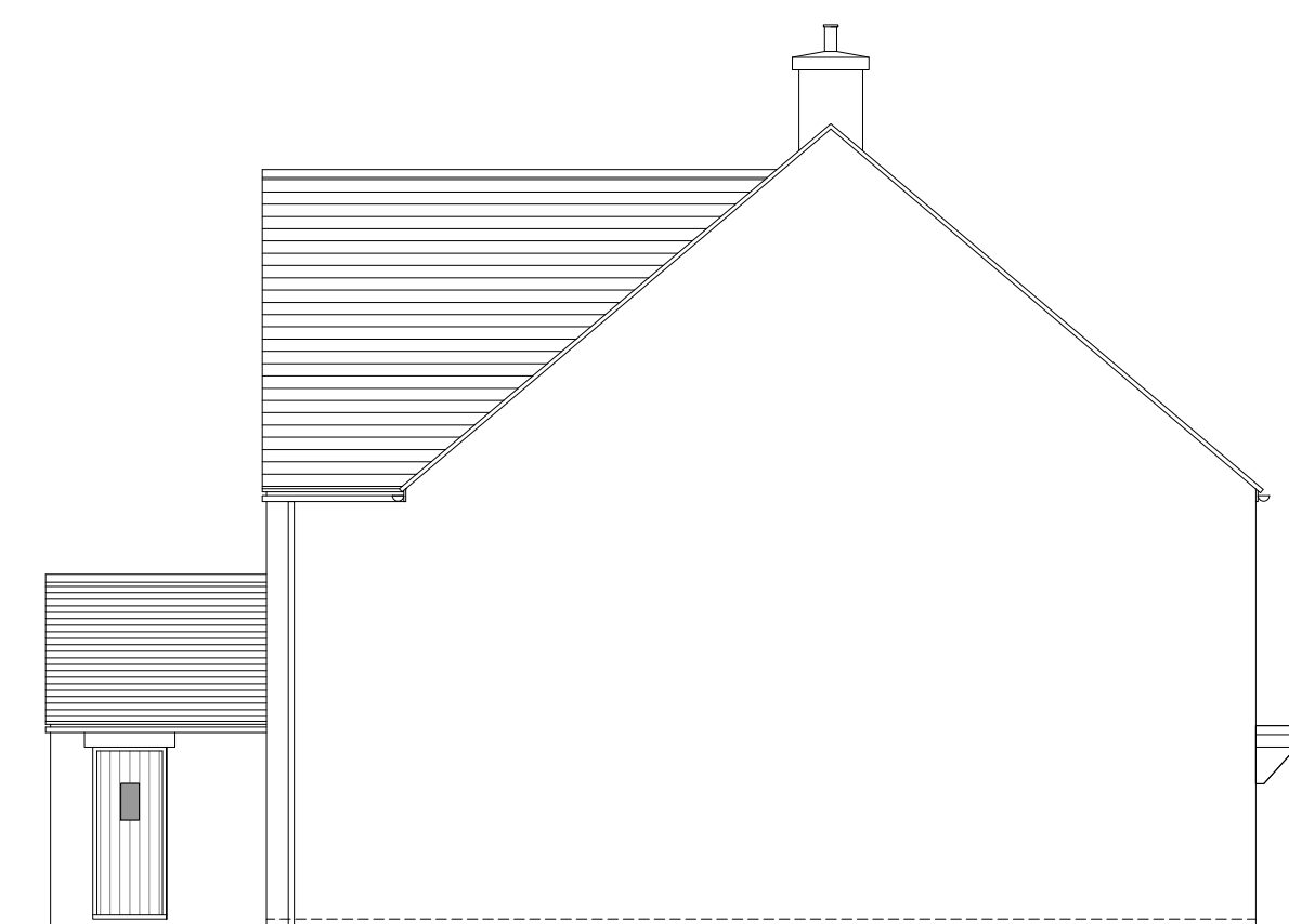
Side Elevation
