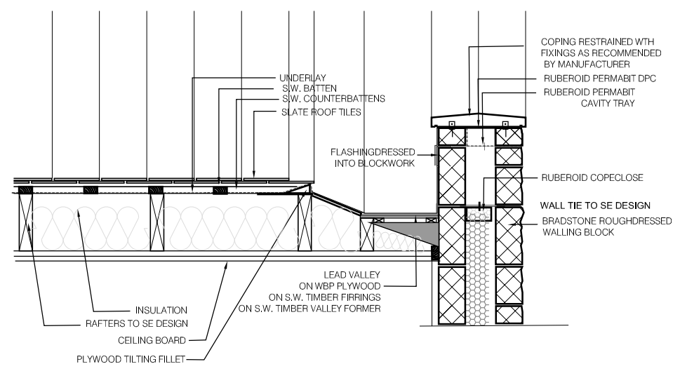
SECTION THROUGH VERGE/COPING
