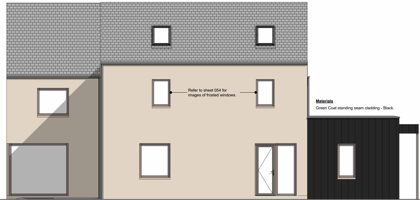
East Elevation 1 : 100
