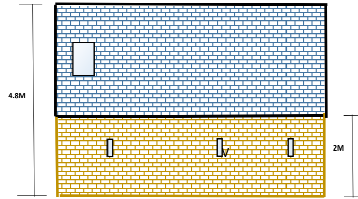
NORTH ELEVATION
