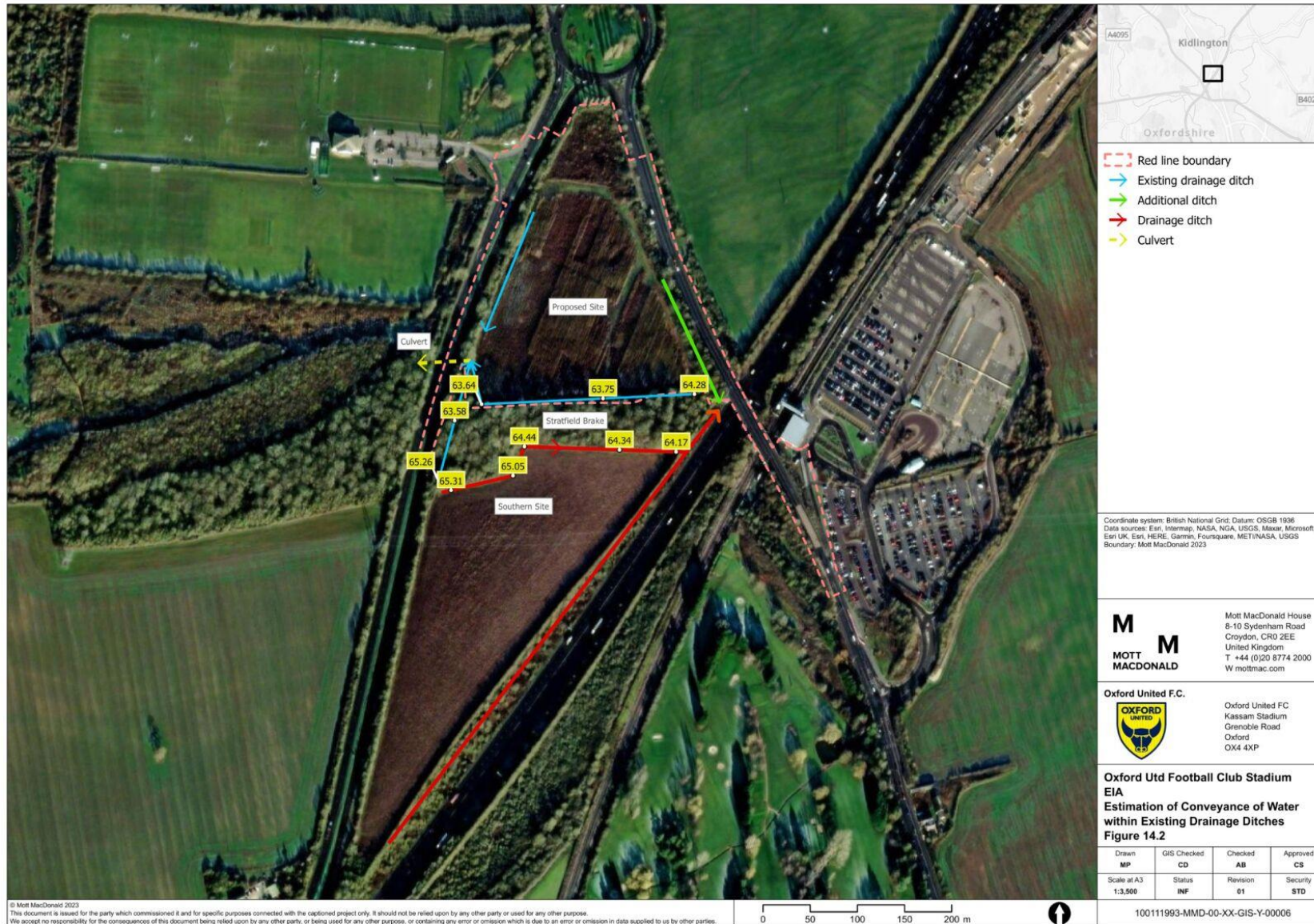
Figure 14.2 - Existing Drainage Ditches
