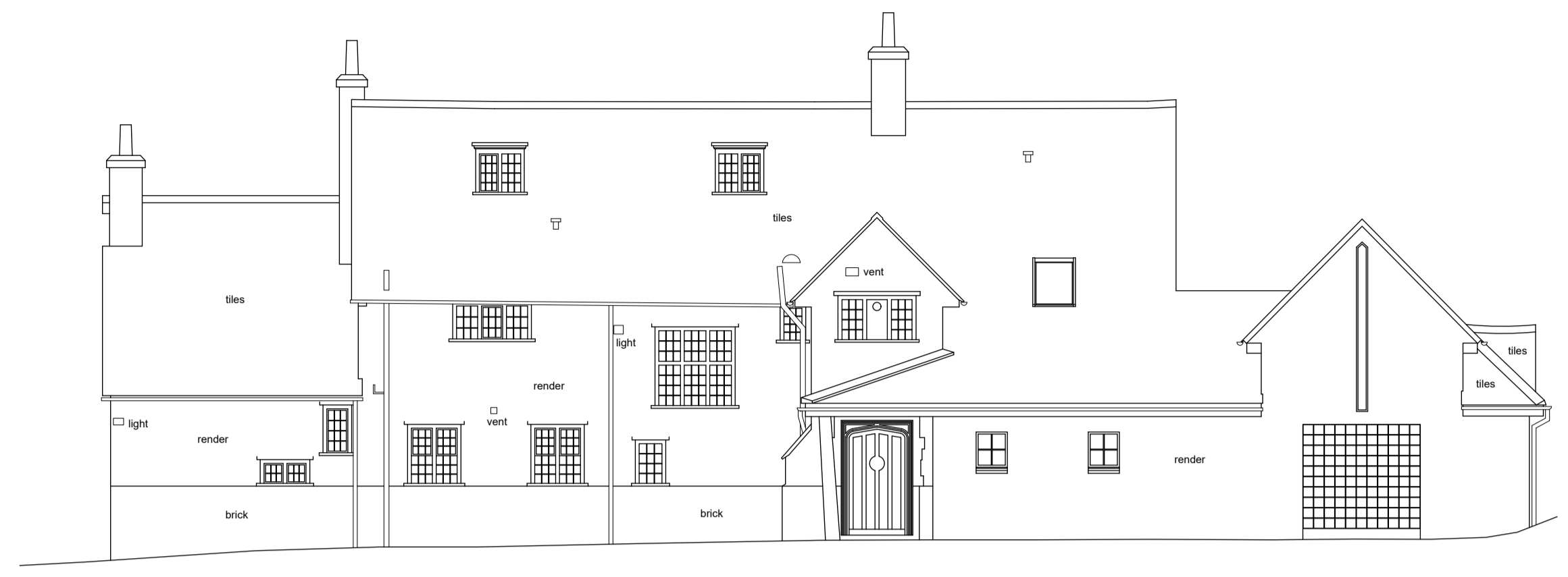
Datum 105.00m NORTH ELEVATION
