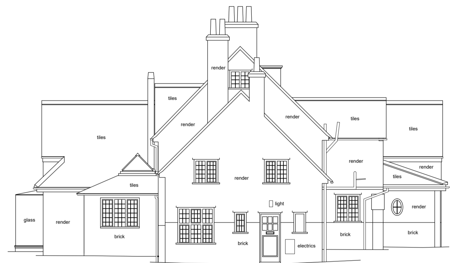
Datum 105.00m EAST ELEVATION
