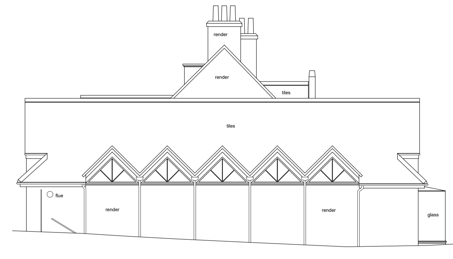
Datum 105.00m WEST ELEVATION
