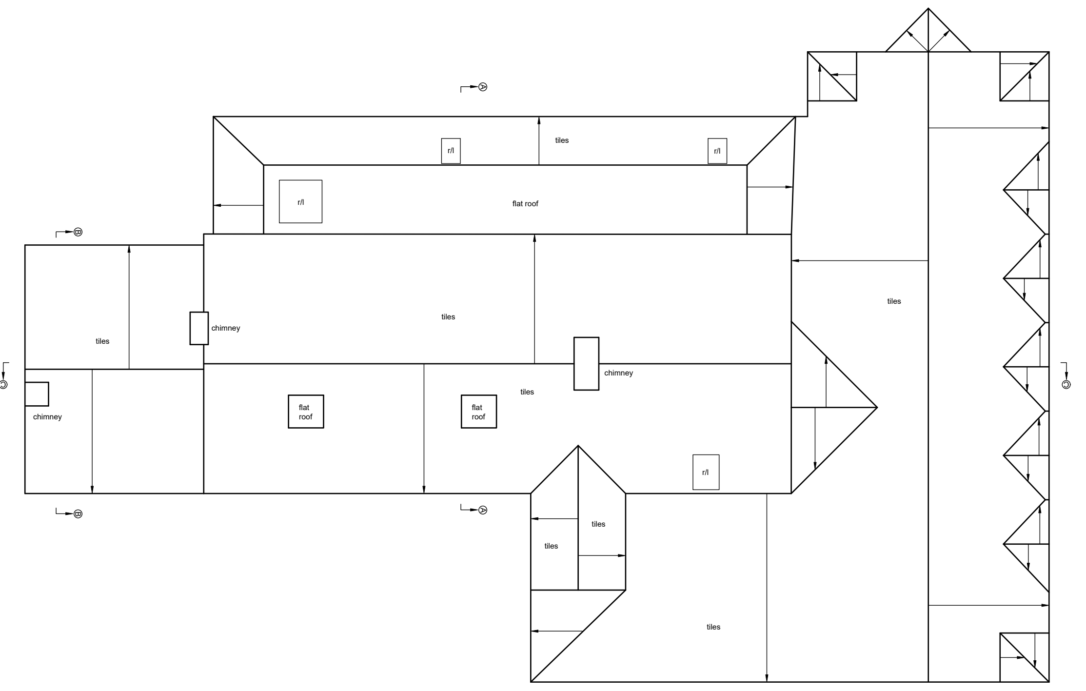
ROOF PLAN
