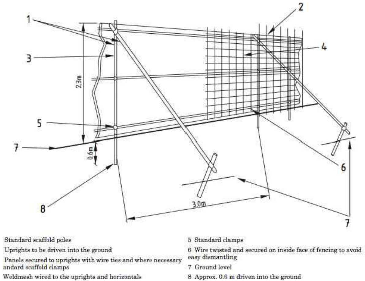
Fig. 2 Protective Barrier Fencing
