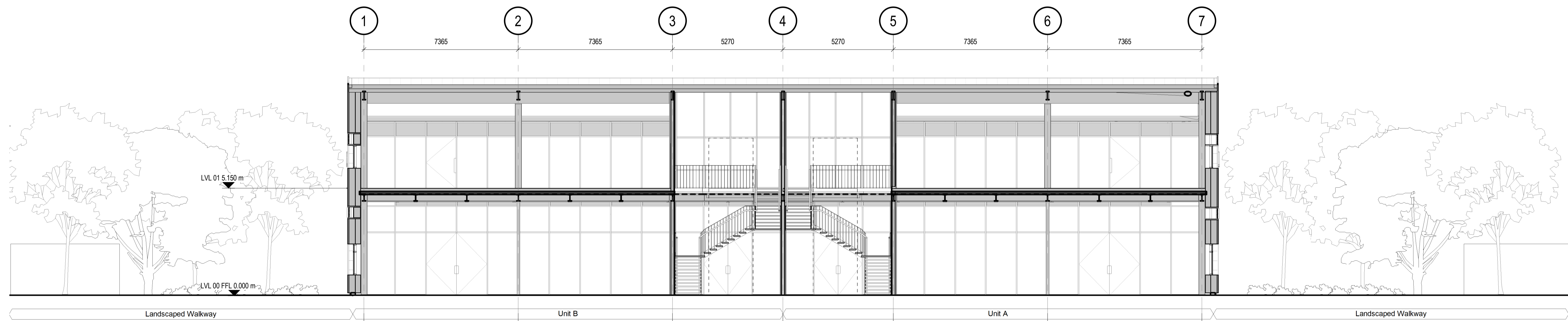
2 Typical building proposed short section DD 1 : 100
