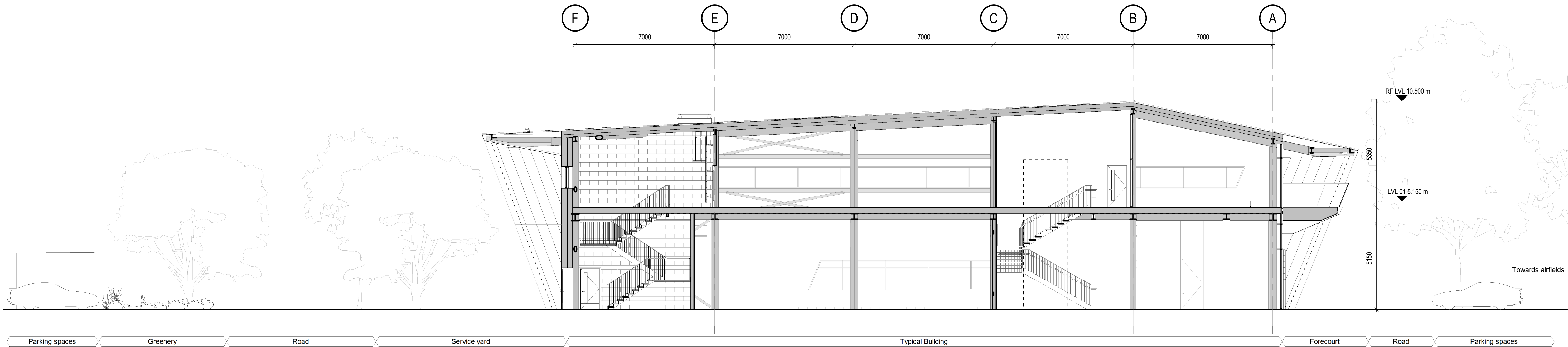
2 Typical building proposed long section BB 1 : 100
