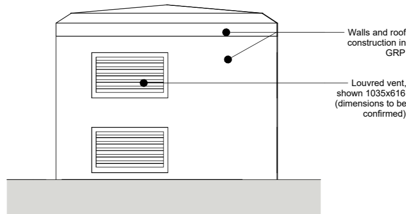
5 Elevation D-Substation 1 : 50
