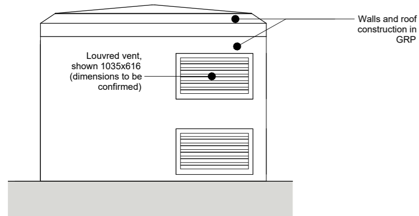
4 Elevation C-Substation 1 : 50
