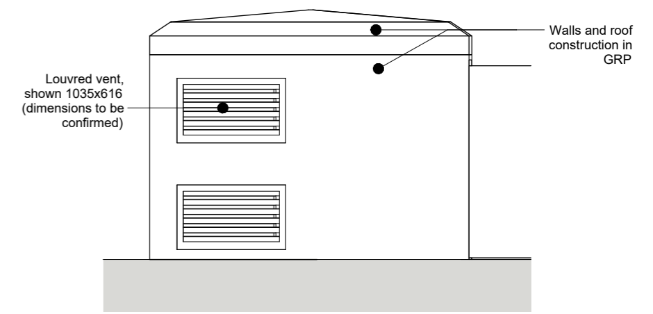
3 Elevation B-Substation 1 : 50
